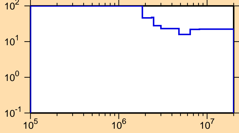
\Delta\sigma/\sigma vs. E for ^{197}\text{Po}(n,n_1)
