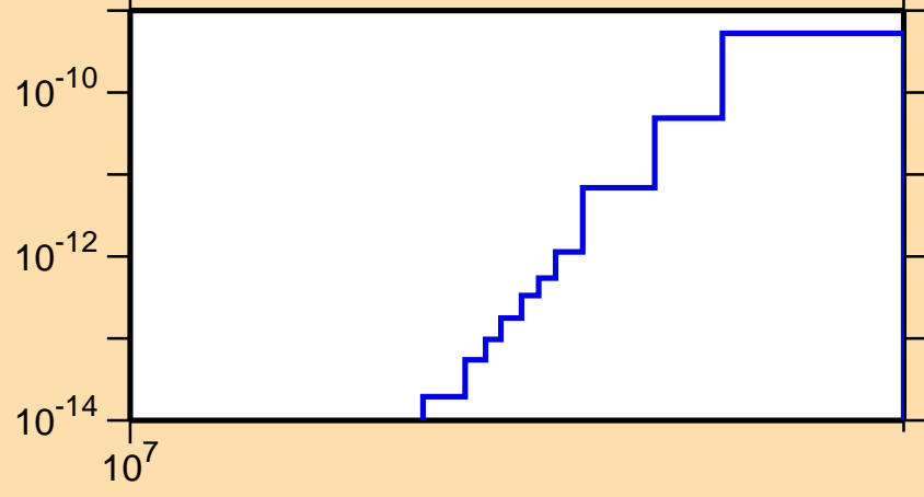
\sigma vs. E for ^{197}\text{Po} (mt 34)
