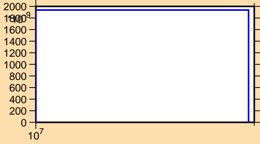
\sigma vs. E for ^{197}\text{Po}(n,2np)
