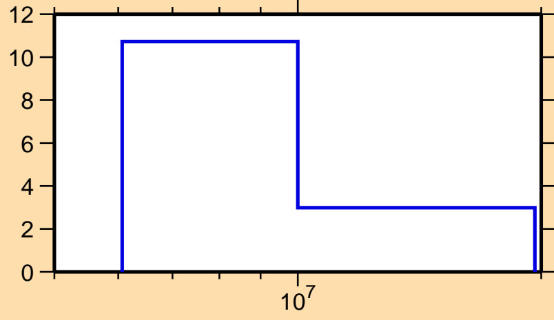
\Delta\sigma/\sigma vs. E for ^{197}\text{Po}(n,\text{tot.})
