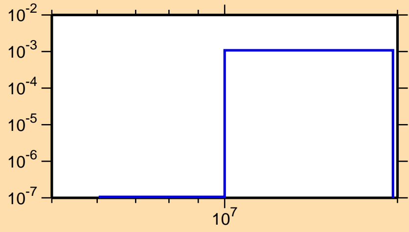
\sigma vs. E for ^{197}\text{Po}(n,2n\alpha)
