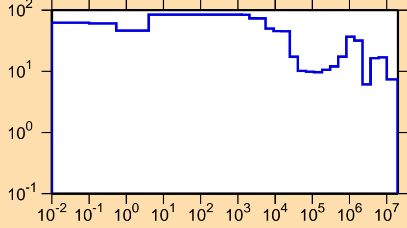
\Delta\sigma/\sigma vs. E for ^{197}\text{Po}(n,\text{el.})
