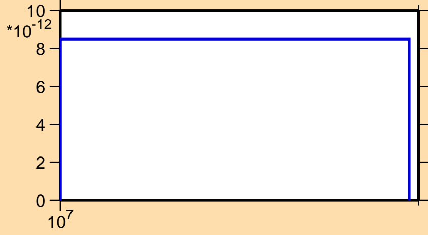
\sigma vs. E for ^{197}\text{Po} (mt 34)
