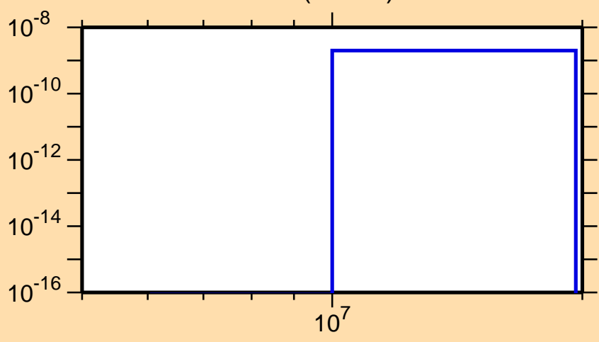
\sigma vs. E for ^{197}\text{Po}(\text{mt } 45)
