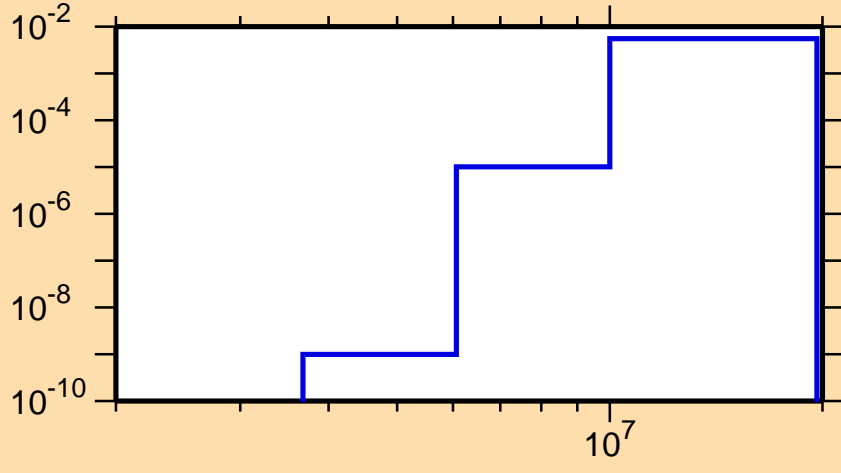
\sigma vs. E for ^{197}\text{Po}(n,d)
