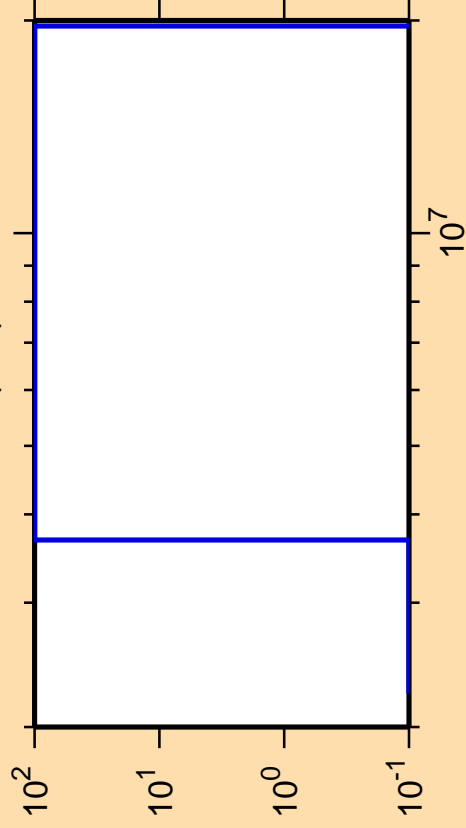
\Delta\sigma/\sigma vs. E for ^{197}\text{Po}(n,d)
