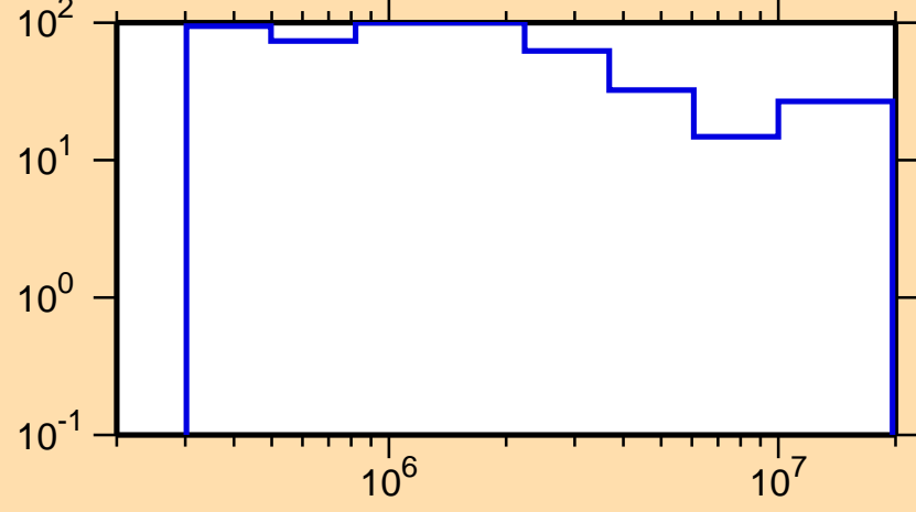
\Delta\sigma/\sigma vs. E for ^{197}\text{Po}(n,n\text{cont.})
