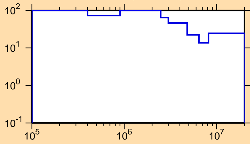
\Delta\sigma/\sigma vs. E for ^{197}\text{Po}(n,n\text{cont.})
