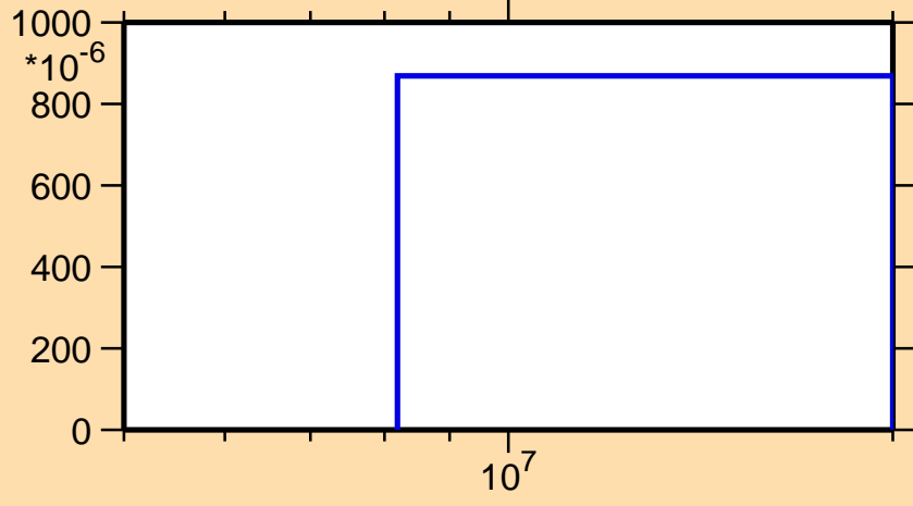
\sigma vs. E for ^{197}\text{Po}(n,2n\alpha)
