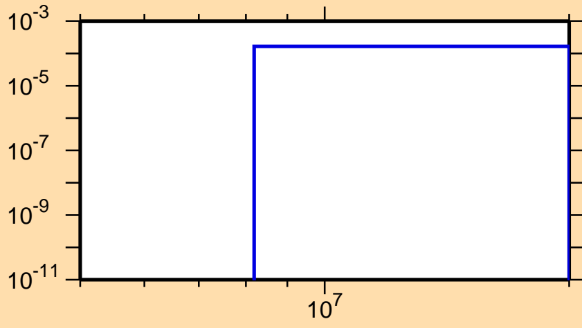
\sigma vs. E for ^{197}\text{Po}(n,t)
