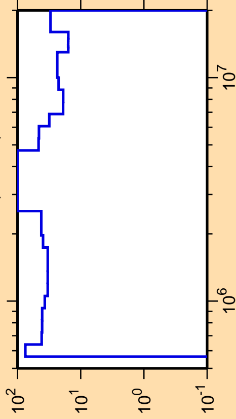
\Delta\sigma/\sigma vs. E for ^{198}\text{Po}(n,\text{inel.})
