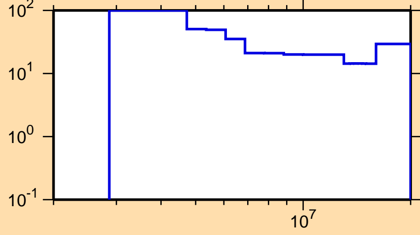
\Delta\sigma/\sigma vs. E for ^{198}\text{Po}(n,n\text{cont.})
