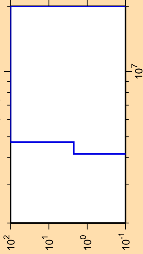
\Delta\sigma/\sigma vs. E for ^{198}\text{Po}(n,d)
