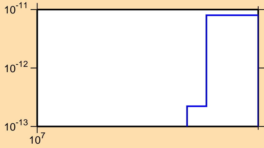
\sigma vs. E for ^{198}\text{Po} (mt 34)
