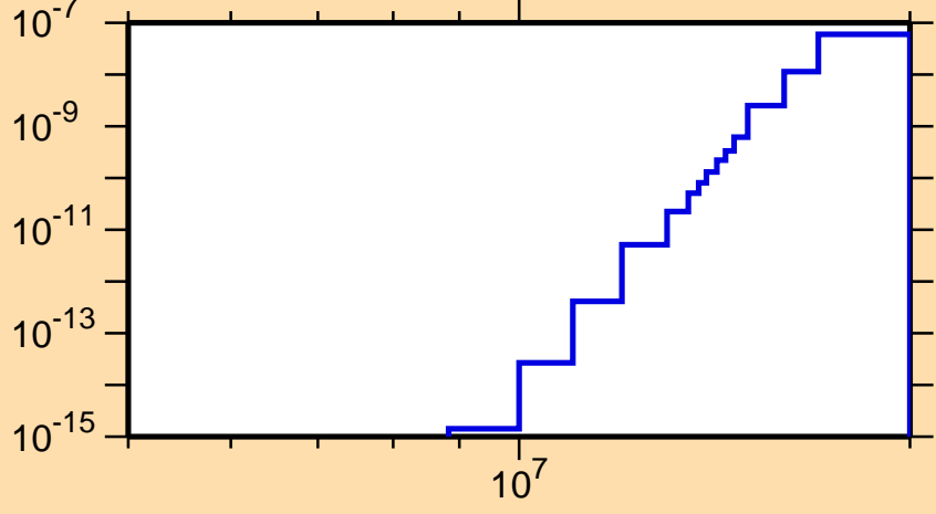
\sigma vs. E for ^{198}\text{Po} (mt 45)
