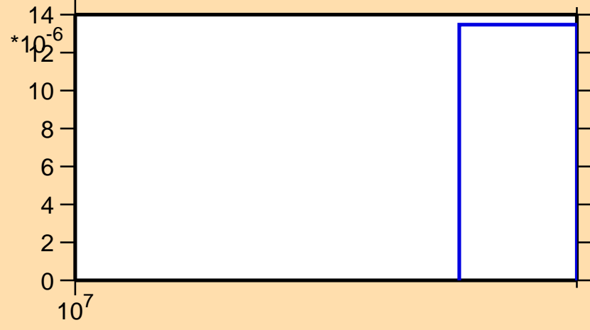
\sigma vs. E for ^{198}\text{Po}(n,3n)
