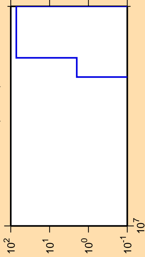
\Delta\sigma/\sigma vs. E for ^{198}\text{Po} (mt 34)
