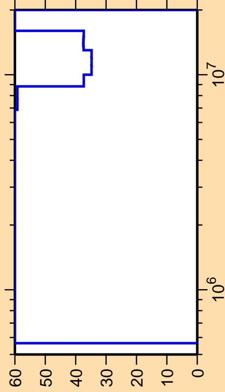
\Delta\sigma/\sigma vs. E for ^{198}\text{Po}(n,p)
