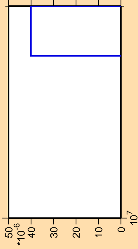
\Delta\sigma/\sigma vs. E for ^{198}\text{Po} (mt 11)
