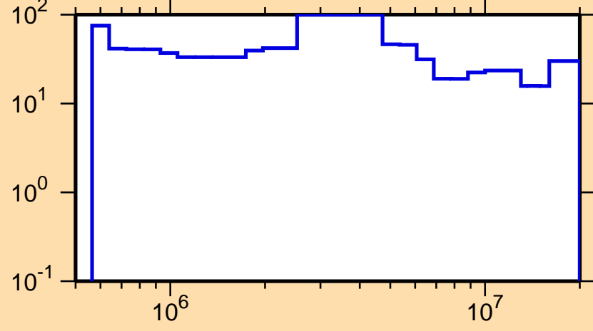
\Delta\sigma/\sigma vs. E for ^{198}\text{Po}(n,\text{inel.})
