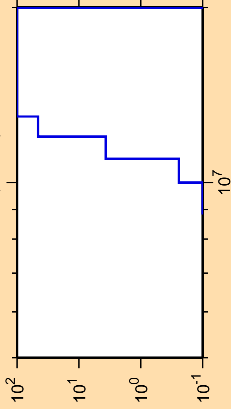
\Delta\sigma/\sigma vs. E for ^{198}\text{Po} (mt 45)
