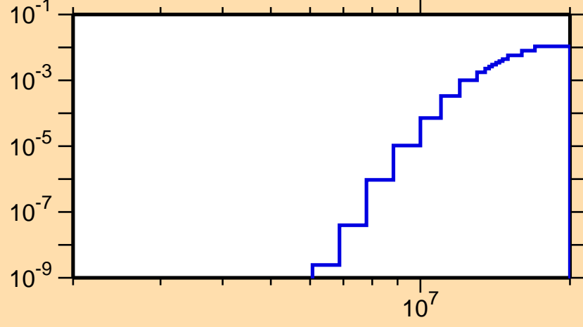
\sigma vs. E for ^{198}\text{Po}(n,d)
