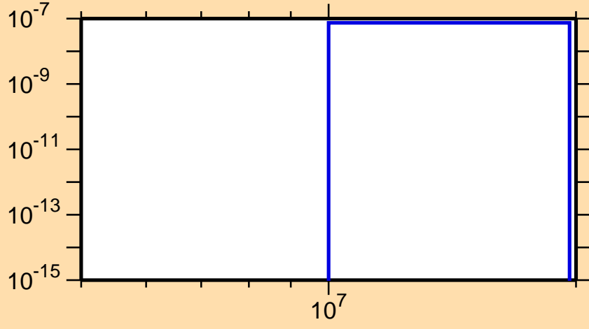
\sigma vs. E for ^{198}\text{Po}(n,2n\alpha)
