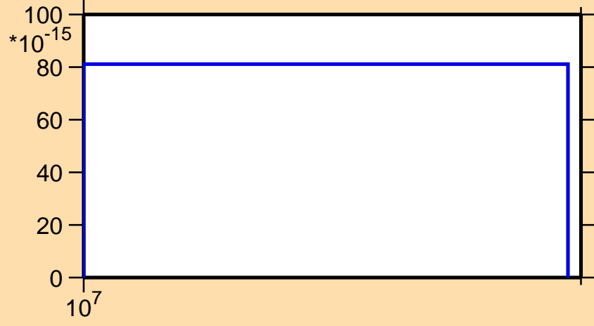
\sigma vs. E for ^{198}\text{Po} (mt 34)
