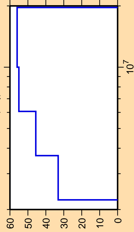
\Delta\sigma/\sigma vs. E for ^{198}\text{Po}(n,\gamma)
