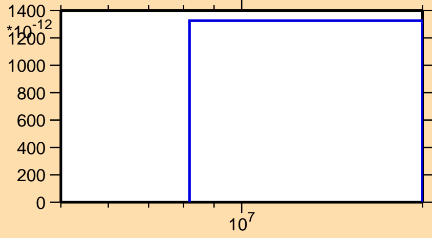
\sigma vs. E for ^{198}\text{Po}(\text{mt } 45)
