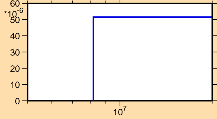
\sigma vs. E for ^{198}\text{Po}(n,t)
