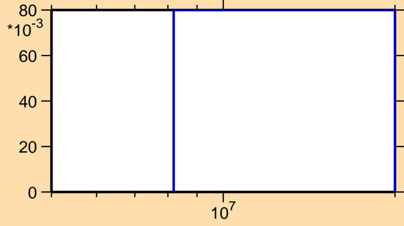
\sigma vs. E for ^{198}\text{Po}(n,2n)
