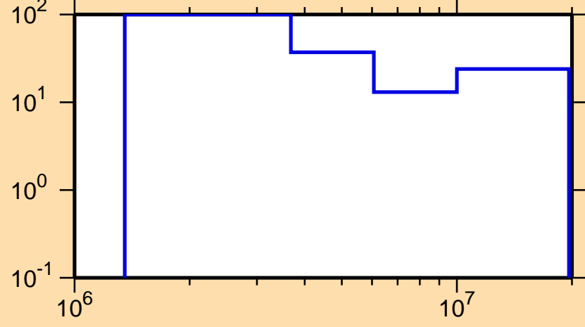
\Delta\sigma/\sigma vs. E for ^{199}\text{Po}(n,n\text{cont.})
