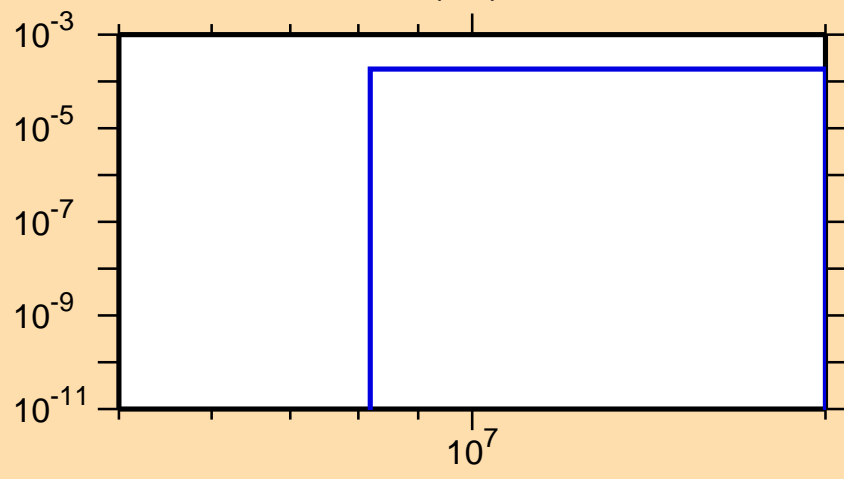
\sigma vs. E for ^{199}\text{Po}(n,t)
