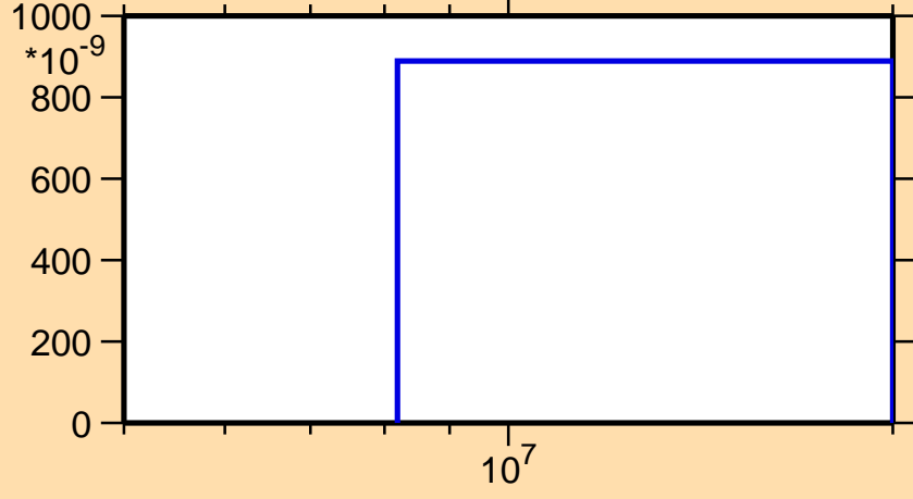
\sigma vs. E for ^{199}\text{Po}(n,2n\alpha)
