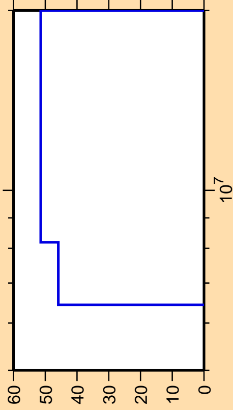
\Delta\sigma/\sigma vs. E for ^{199}\text{Po}(n,\gamma)
