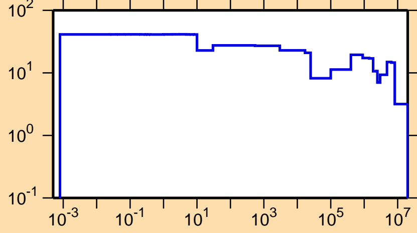
\Delta\sigma/\sigma vs. E for ^{199}\text{Po}(n,\text{el.})
