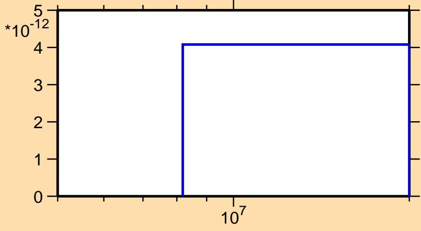
\sigma vs. E for ^{199}\text{Po} (mt 34)
