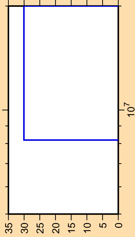
\Delta\sigma/\sigma vs. E for ^{199}\text{Po} (mt 34)
