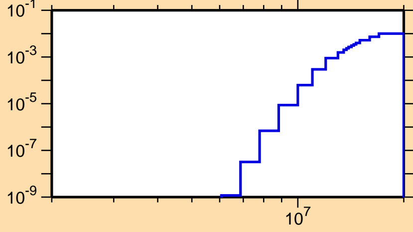
\sigma vs. E for ^{199}\text{Po}(n,d)
