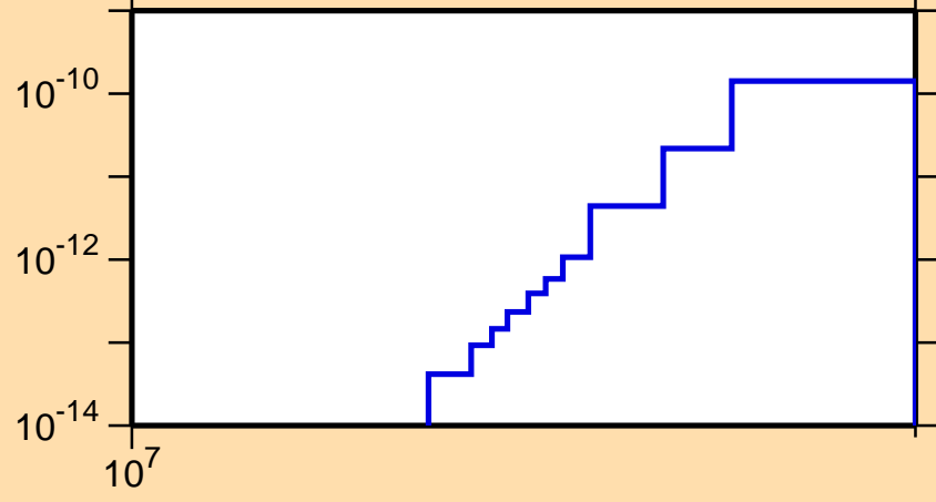
\sigma vs. E for ^{199}\text{Po}(\text{mt117})
