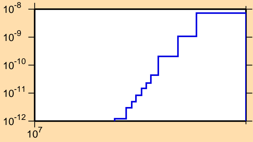
\sigma vs. E for ^{199}\text{Po}(\text{mt } 45)
