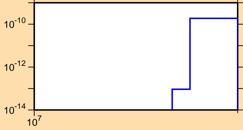
\sigma vs. E for ^{199}\text{Po}(n,nt)
