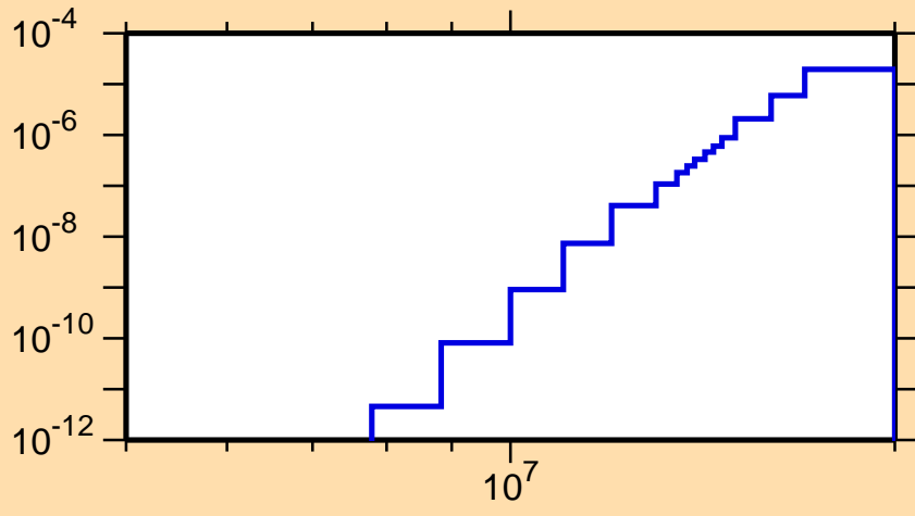
\sigma vs. E for ^{199}\text{Po}(n,\text{He3})
