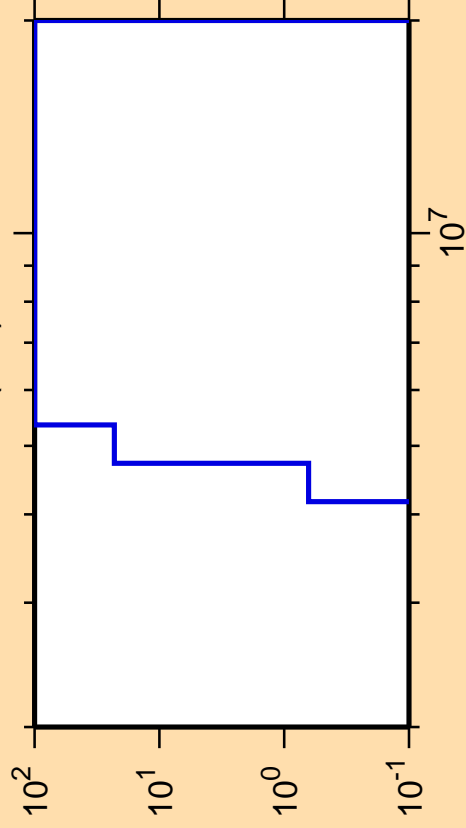
\Delta\sigma/\sigma vs. E for ^{199}\text{Po}(n,d)
