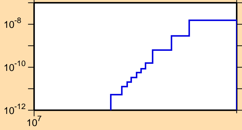
\sigma vs. E for ^{199}\text{Po}(n,\text{pd})
