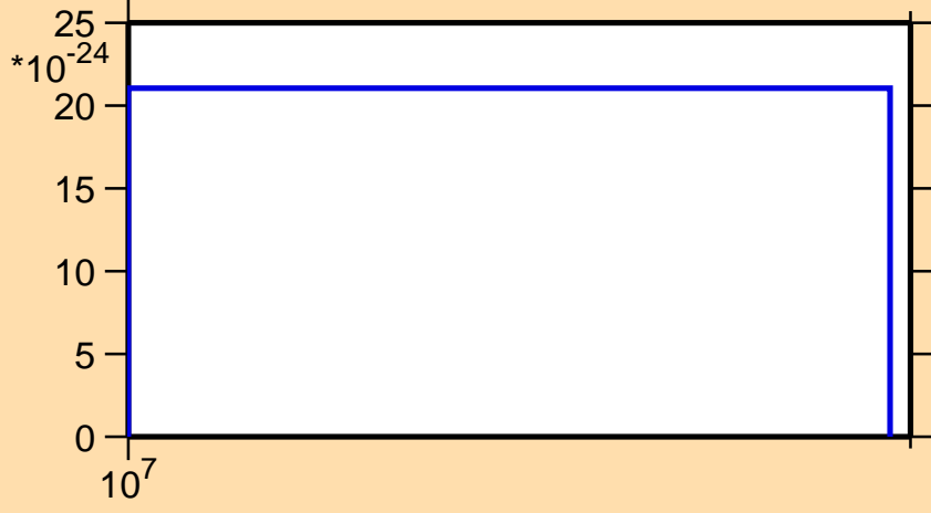
\sigma vs. E for ^{199}\text{Po} (mt 11)
