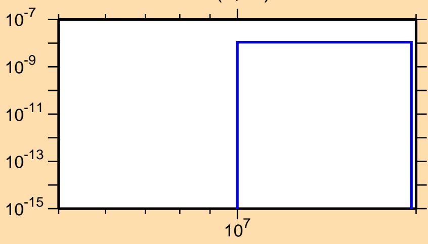
\sigma vs. E for ^{199}\text{Po}(n,\text{nd})
