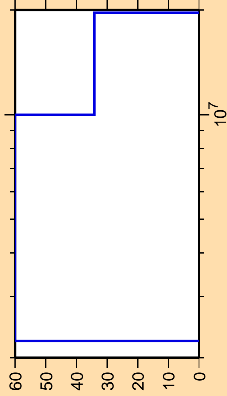
\Delta\sigma/\sigma vs. E for ^{200}\text{Po}(n,p)
