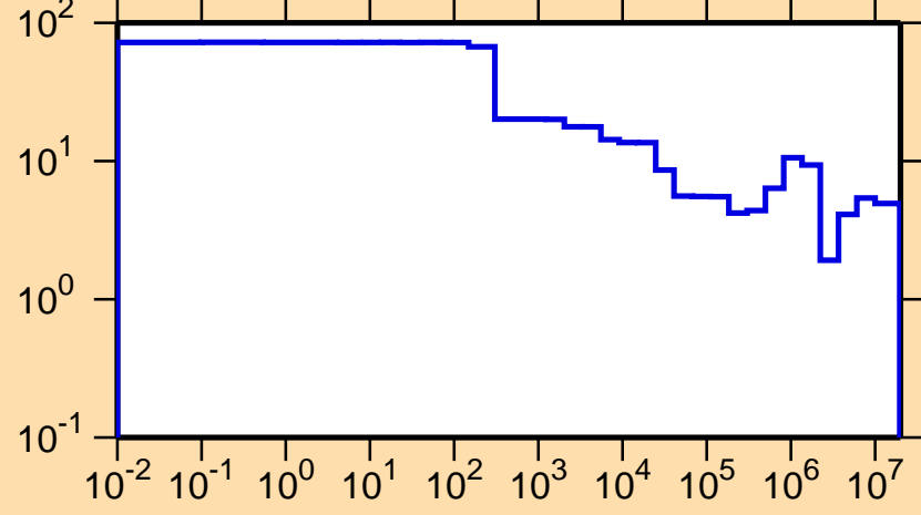
\Delta\sigma/\sigma vs. E for ^{200}\text{Po}(n,\text{el.})
