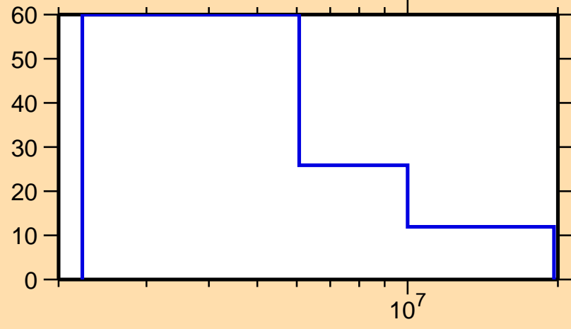
\Delta\sigma/\sigma vs. E for ^{200}\text{Po}(n,ncont.)
