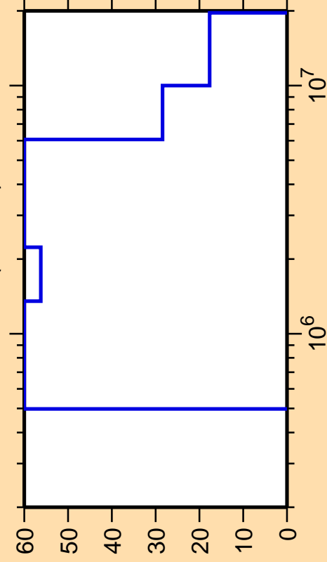
\Delta\sigma/\sigma vs. E for ^{200}\text{Po}(n,\text{inel.})
