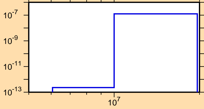
\sigma vs. E for ^{200}\text{Po}(n,\text{He3})
