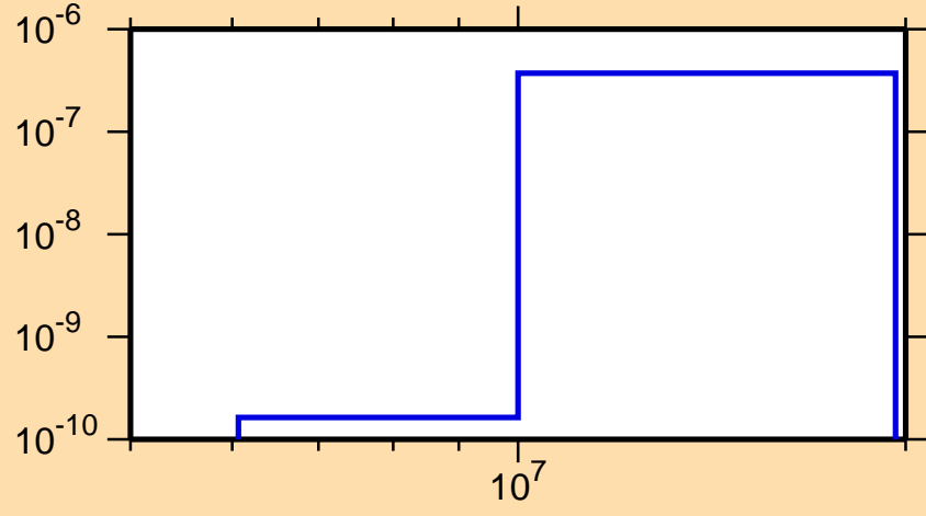
\sigma vs. E for ^{200}\text{Po}(n,p\alpha)
