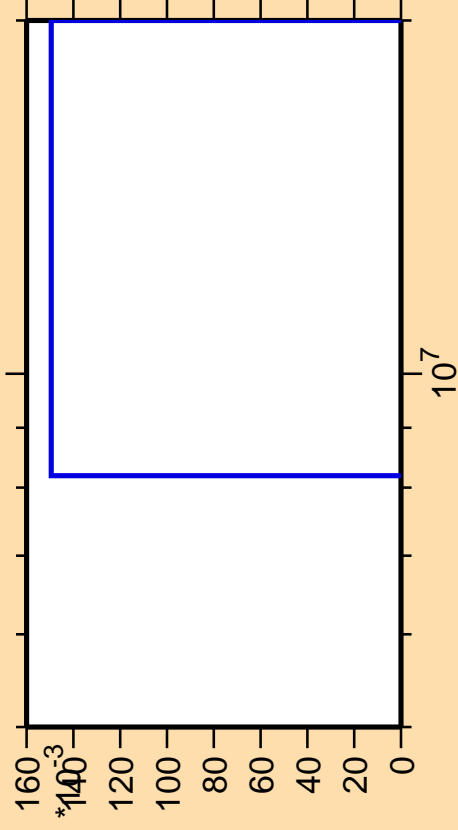
\Delta\sigma/\sigma vs. E for ^{200}\text{Po} (mt 34)
