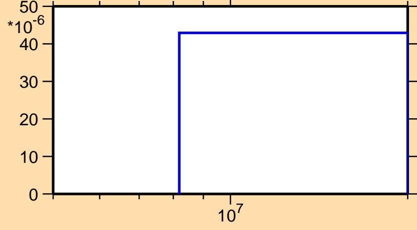
\sigma vs. E for ^{200}\text{Po}(n,t)
