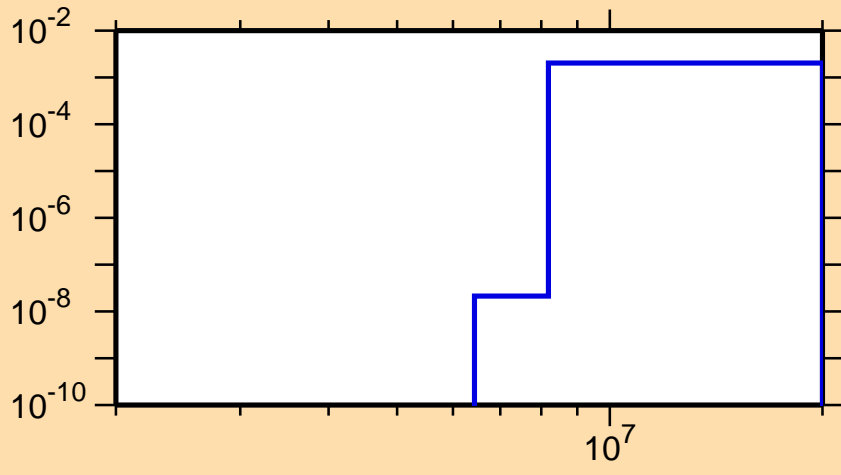
\sigma vs. E for ^{200}\text{Po}(n,d)
