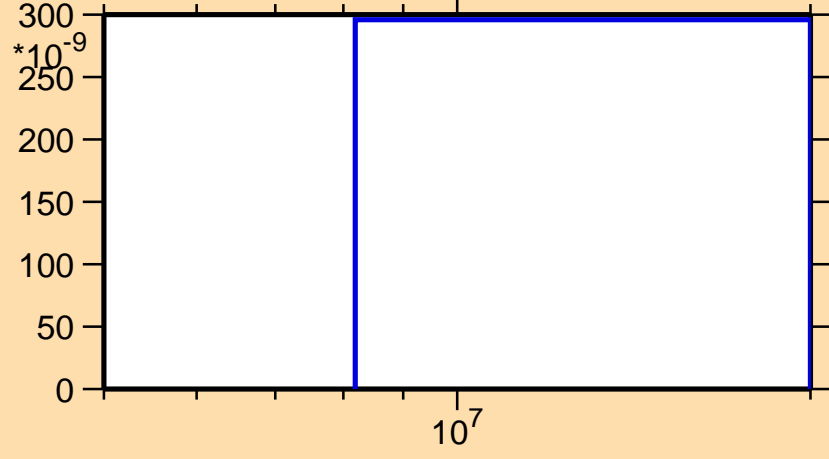
\sigma vs. E for ^{200}\text{Po}(n,3n)
