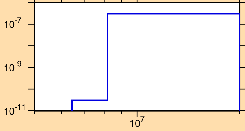
\sigma vs. E for ^{200}\text{Po}(n,p\alpha)
