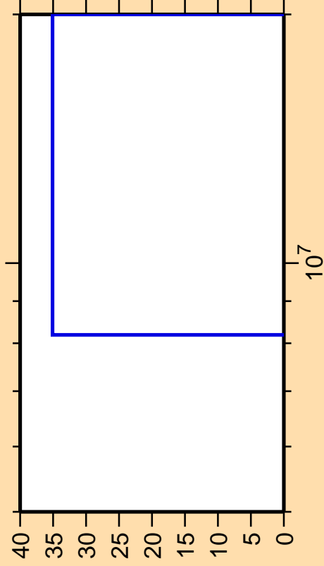
\Delta\sigma/\sigma vs. E for ^{200}\text{Po} (mt 45)
