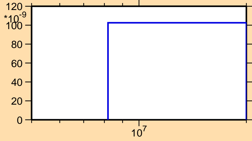
\sigma vs. E for ^{200}\text{Po}(n,\text{He}3)
