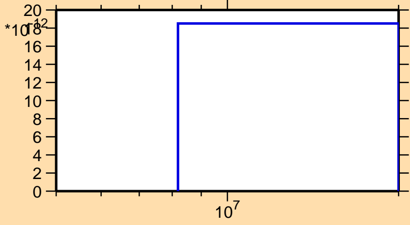
\sigma vs. E for ^{200}\text{Po} (mt 45)
