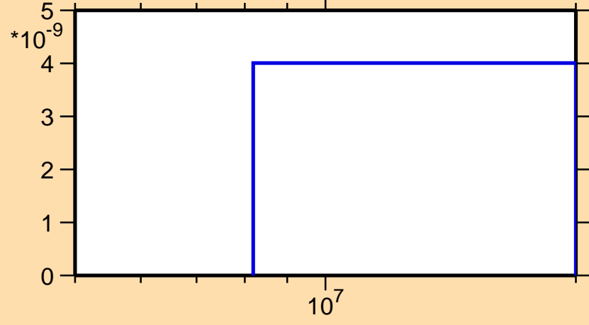
\sigma vs. E for ^{200}\text{Po}(n,2np)
