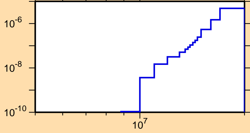
\sigma vs. E for ^{201}\text{Po}(n,2n\alpha)
