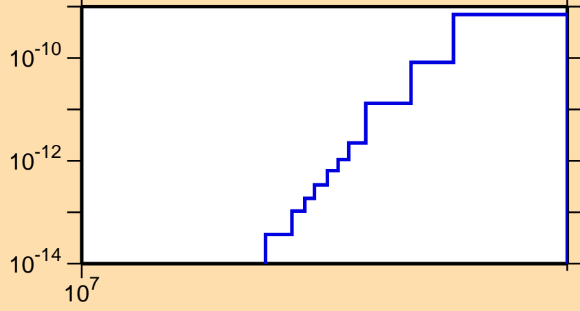
\sigma vs. E for ^{201}\text{Po}(\text{mt } 45)
