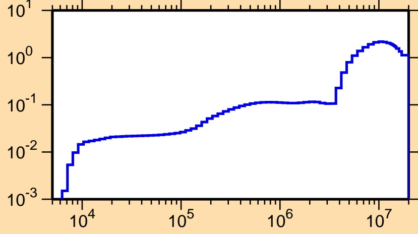
\sigma vs. E for ^{201}\text{Po}(n,\text{inel.})
