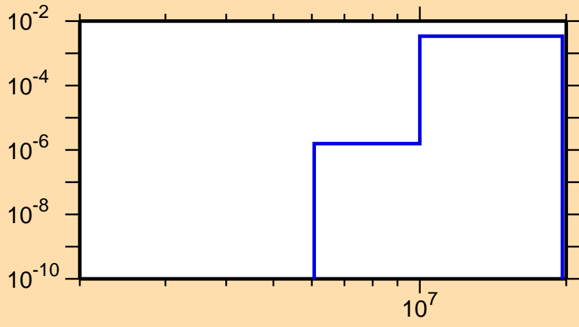
\sigma vs. E for ^{201}\text{Po}(n,d)
