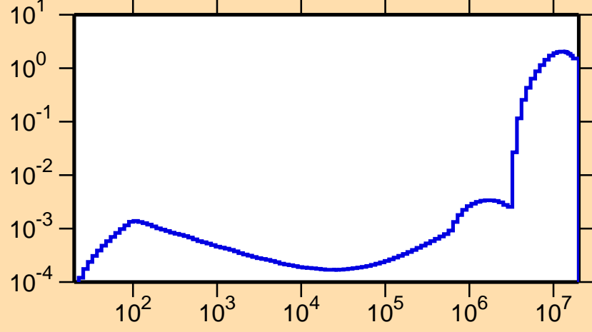
\sigma vs. E for ^{201}\text{Po}(n,\text{inel.})
