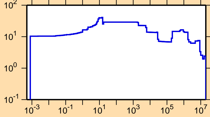
\Delta\sigma/\sigma vs. E for ^{201}\text{Po}(n,\text{tot.})
