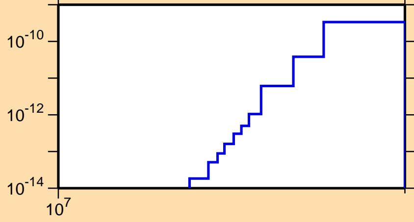
\sigma vs. E for ^{201}\text{Po} (mt 45)
