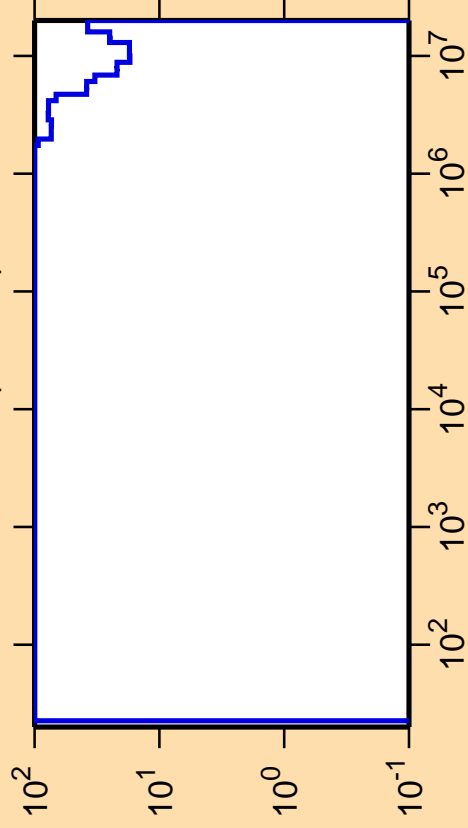
\Delta\sigma/\sigma vs. E for ^{201}\text{Po}(n,\text{inel.})
