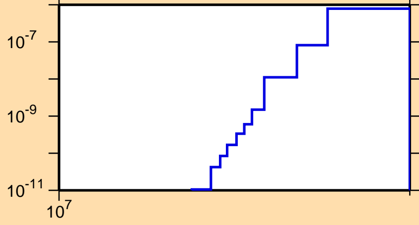
\sigma vs. E for ^{201}\text{Po}(n,\text{nd})
