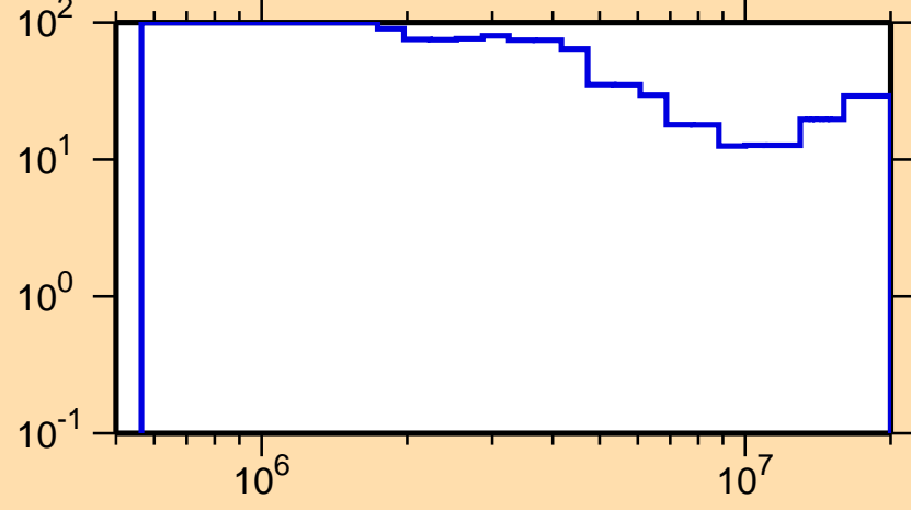
\Delta\sigma/\sigma vs. E for ^{201}\text{Po}(n,n\text{cont.})
