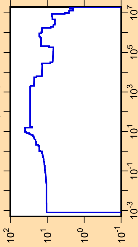
\Delta\sigma/\sigma vs. E for ^{201}\text{Po}(n,\text{tot.})
