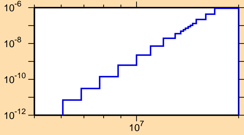
\sigma vs. E for ^{201}\text{Po}(n,p\alpha)
