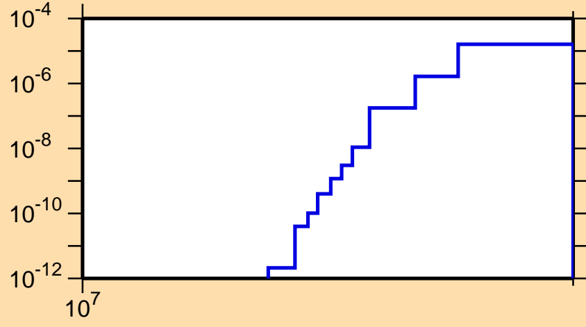
\sigma vs. E for ^{201}\text{Po}(n,2np)
