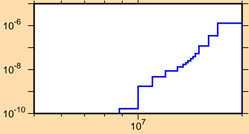
\sigma vs. E for ^{201}\text{Po}(n,2n\alpha)
