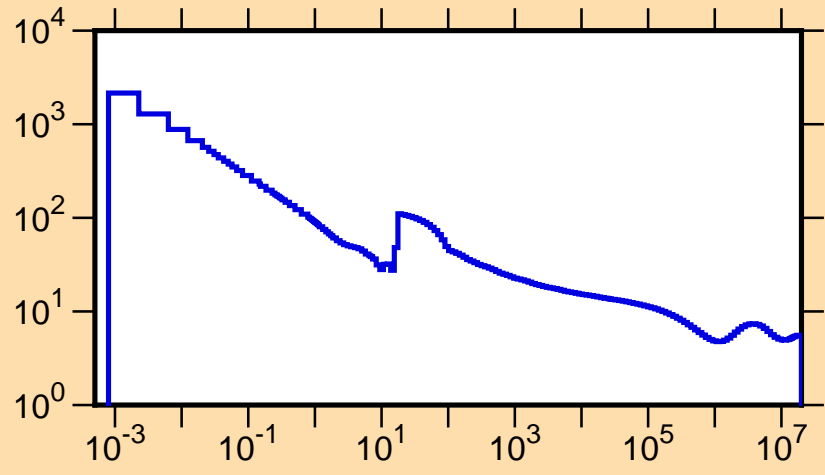
\sigma vs. E for ^{201}\text{Po}(n,\text{tot.})
