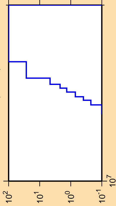
\Delta\sigma/\sigma vs. E for ^{201}\text{Po} (mt 45)
