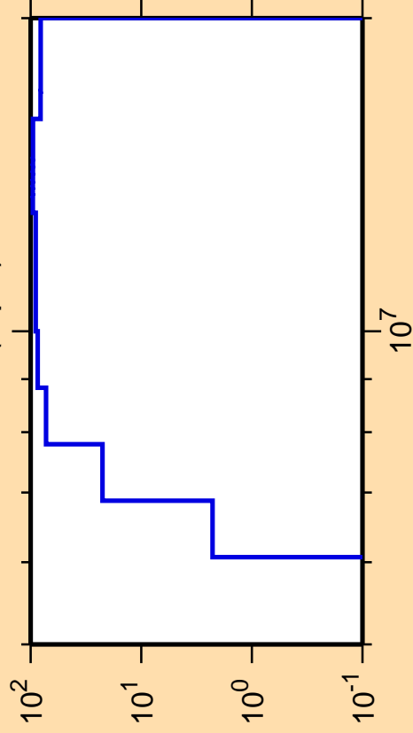
\Delta\sigma/\sigma vs. E for ^{201}\text{Po}(n,p\alpha)
