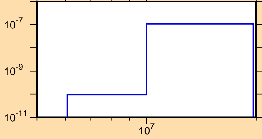
\sigma vs. E for ^{201}\text{Po}(n,p\alpha)
