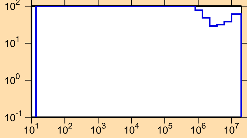
\Delta\sigma/\sigma vs. E for ^{201}\text{Po}(n,n_1)
