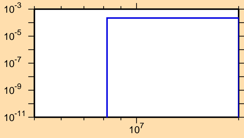
\sigma vs. E for ^{201}\text{Po}(n,t)
