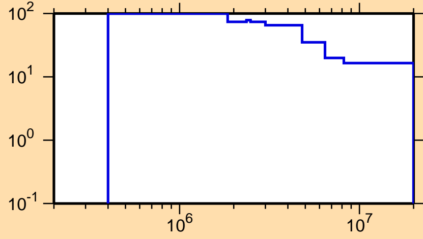
\Delta\sigma/\sigma vs. E for ^{201}\text{Po}(n,n\text{cont.})
