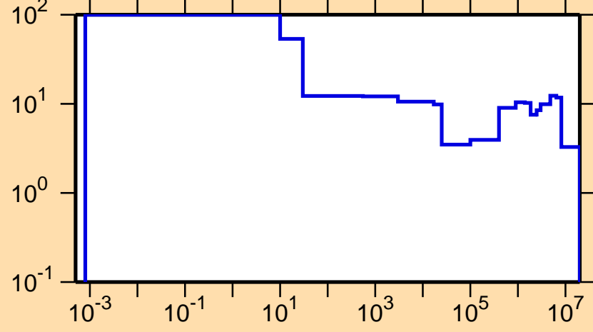
\Delta\sigma/\sigma vs. E for ^{201}\text{Po}(n,\text{el.})
