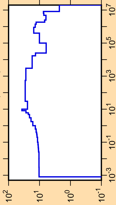
\Delta\sigma/\sigma vs. E for ^{201}\text{Po}(n,\text{tot.})
