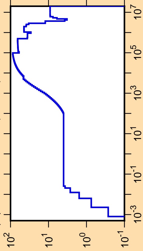
\Delta\mu/\mu vs. E for ^{202}\text{Po}(\text{mt251})
