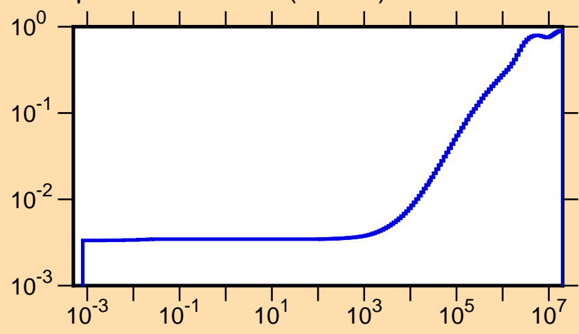
\mu vs. E for ^{202}\text{Po}(\text{mt251})
