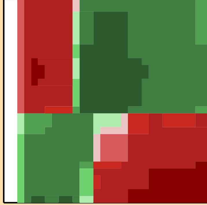
\Delta\sigma/\sigma vs. E for ^{202}\text{Po}(n,n_1)
