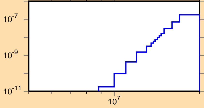
\sigma vs. E for ^{202}\text{Po}(n,p\alpha)
