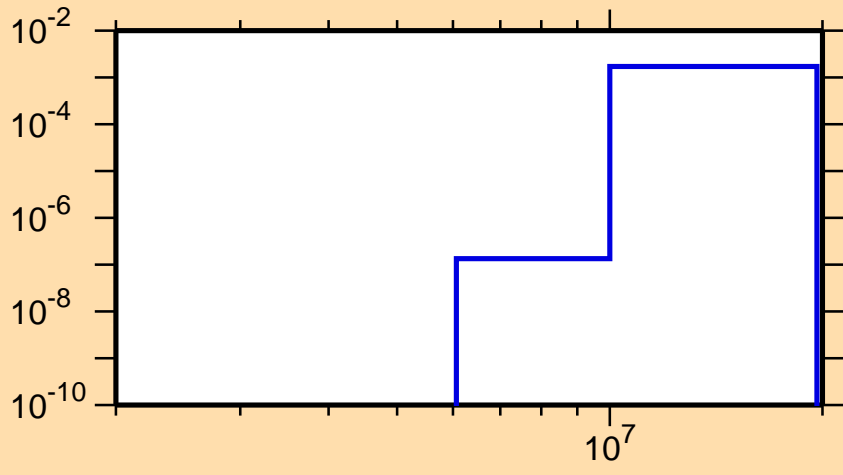
\sigma vs. E for ^{202}\text{Po}(n,d)
