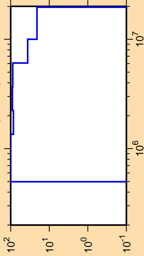
\Delta\sigma/\sigma vs. E for ^{202}\text{Po}(n,\text{inel.})
