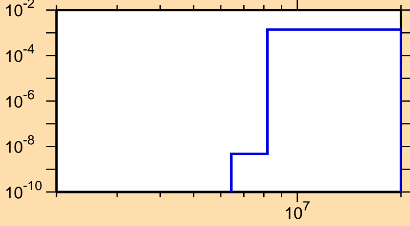
\sigma vs. E for ^{202}\text{Po}(n,d)
