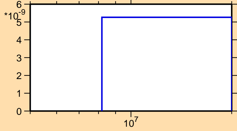
\sigma vs. E for ^{202}\text{Po}(n,2np)
