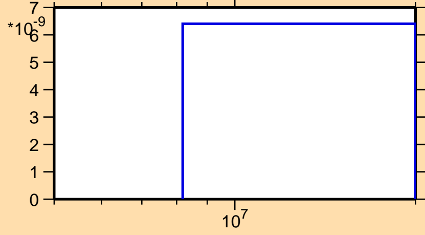
\sigma vs. E for ^{202}\text{Po}(n,2n\alpha)
