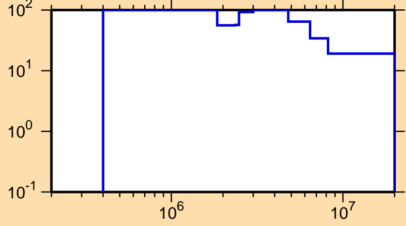
\Delta\sigma/\sigma vs. E for ^{202}\text{Po}(n,\text{inel.})
