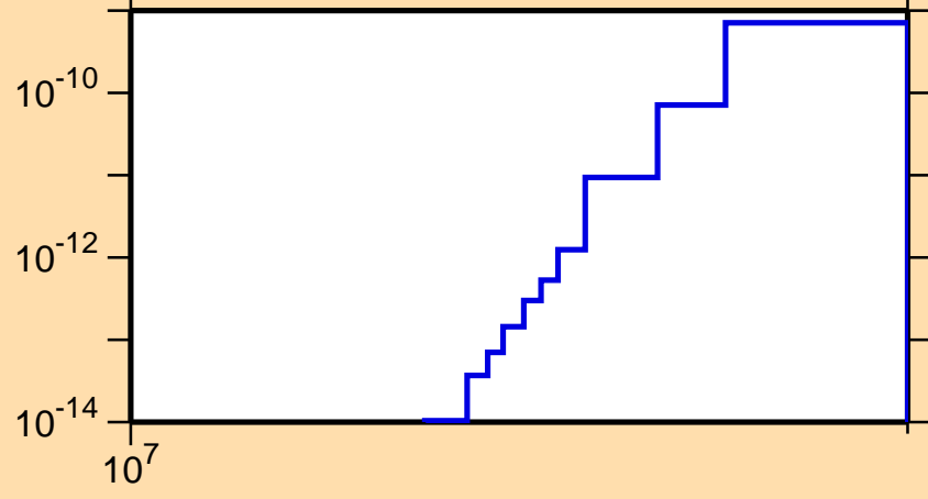
\sigma vs. E for ^{203}\text{Po}(n,\text{pd})
