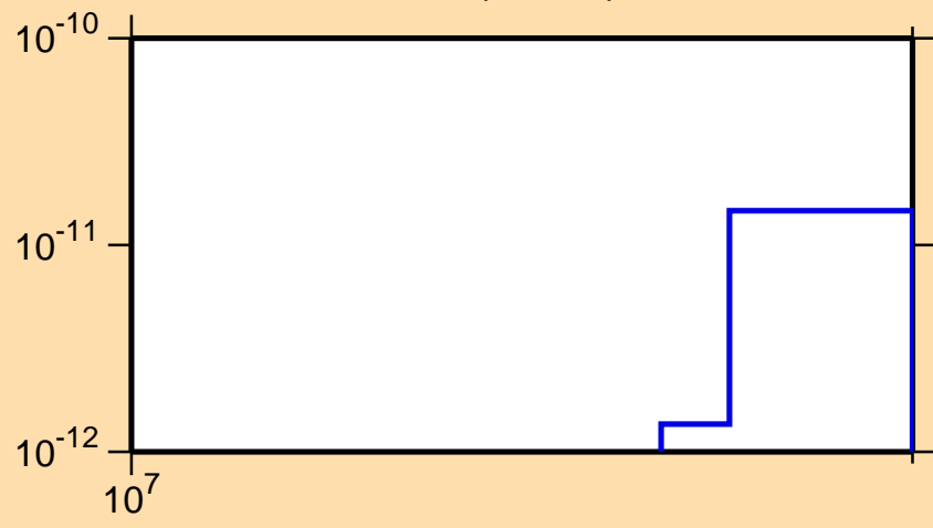
\sigma vs. E for ^{203}\text{Po} (mt 45)
