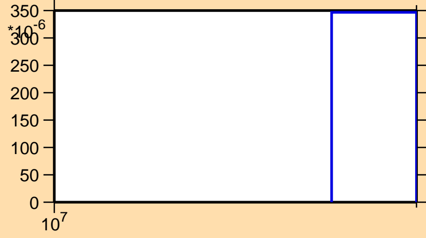
\sigma vs. E for ^{203}\text{Po}(n,3n)
