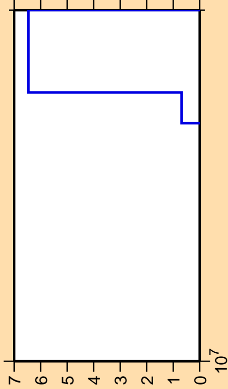
\Delta\sigma/\sigma vs. E for ^{203}\text{Po}(\text{mt117})
