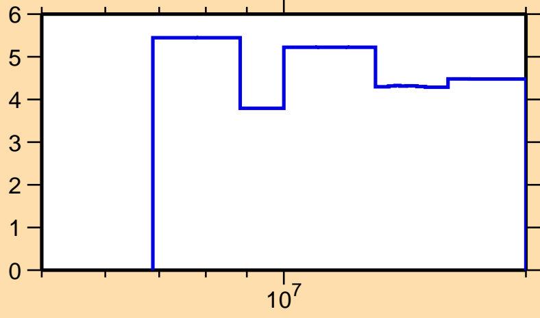
\Delta\sigma/\sigma vs. E for ^{203}\text{Po}(n,tot.)
