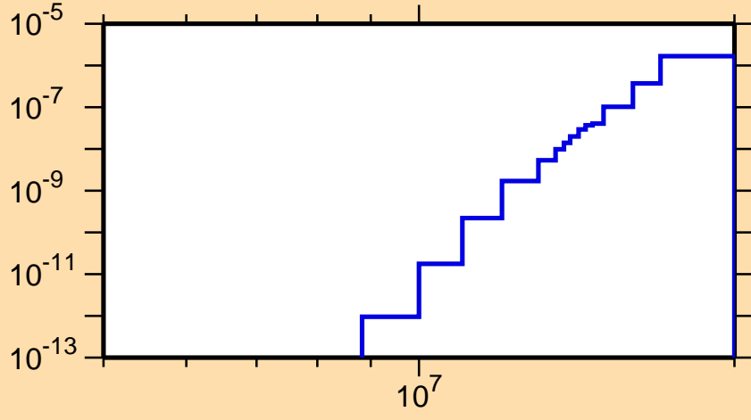
\sigma vs. E for ^{203}\text{Po}(n,\text{He3})
