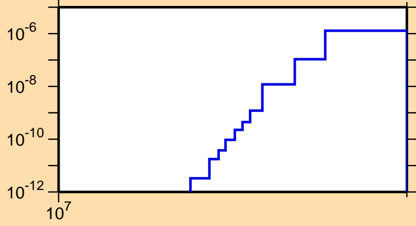
\sigma vs. E for ^{203}\text{Po}(n,\text{nd})
