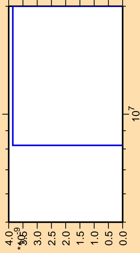
\Delta\sigma/\sigma vs. E for ^{203}\text{Po}(\text{mt 11})
