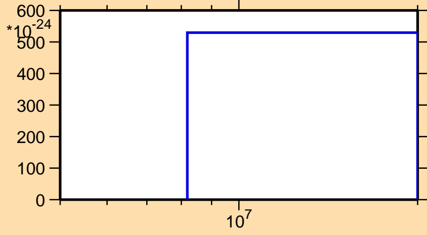
\sigma vs. E for ^{203}\text{Po}(\text{mt 11})
