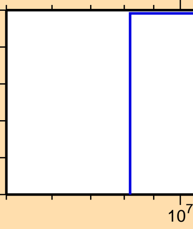
\sigma vs. E for ^{203}\text{Po}(n,\text{pd})
