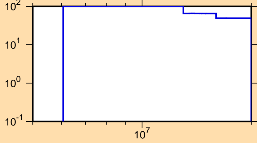
\Delta\sigma/\sigma vs. E for ^{203}\text{Po}(n,2n)
