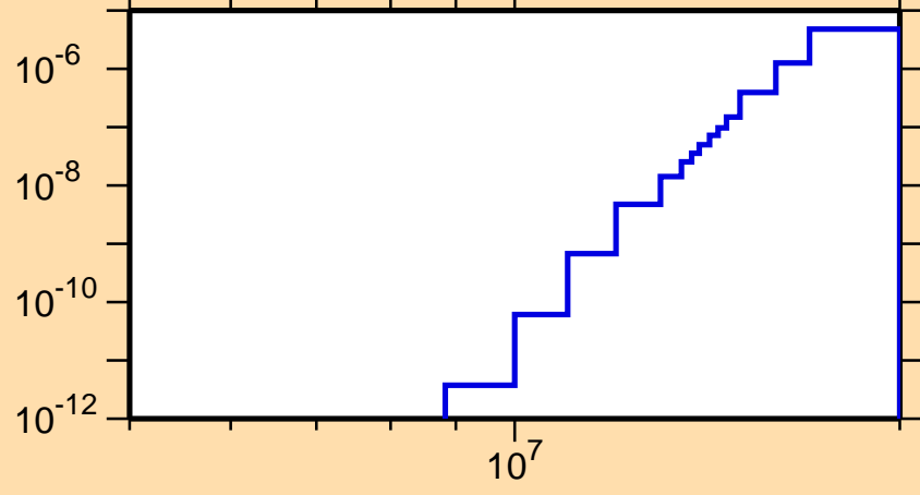
\sigma vs. E for ^{203}\text{Po}(n,\text{He}3)
