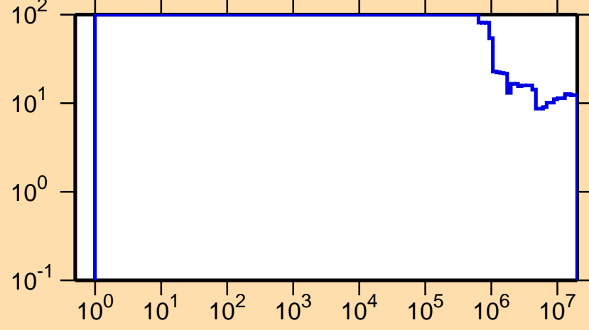
\Delta\sigma/\sigma vs. E for ^{203}\text{Po}(n,n\text{onel.})
