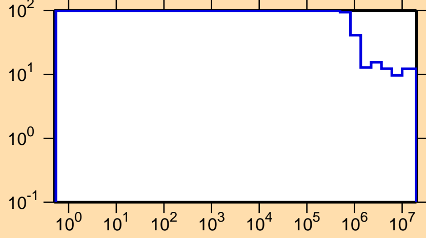
\Delta\sigma/\sigma vs. E for ^{203}\text{Po}(n,n\text{nonel.})
