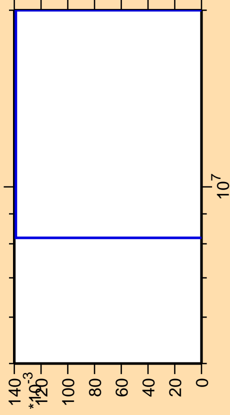
\Delta\sigma/\sigma vs. E for ^{203}\text{Po}(\text{mt117})
