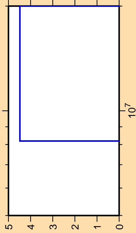
\Delta\sigma/\sigma vs. E for ^{203}\text{Po} (mt 34)
