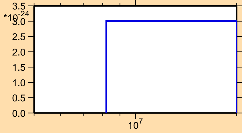
\sigma vs. E for ^{203}\text{Po} (mt 42)
