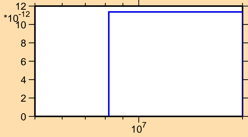
\sigma vs. E for ^{203}\text{Po}(n,\text{pd})
