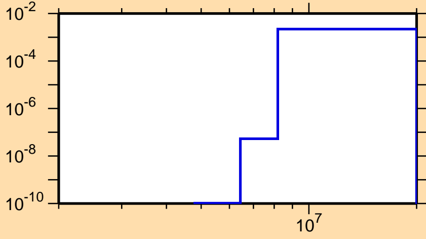
\sigma vs. E for ^{203}\text{Po}(n,d)
