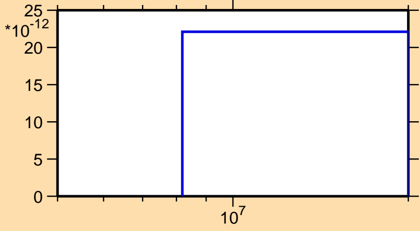
\sigma vs. E for ^{203}\text{Po}(n,\text{nt})
