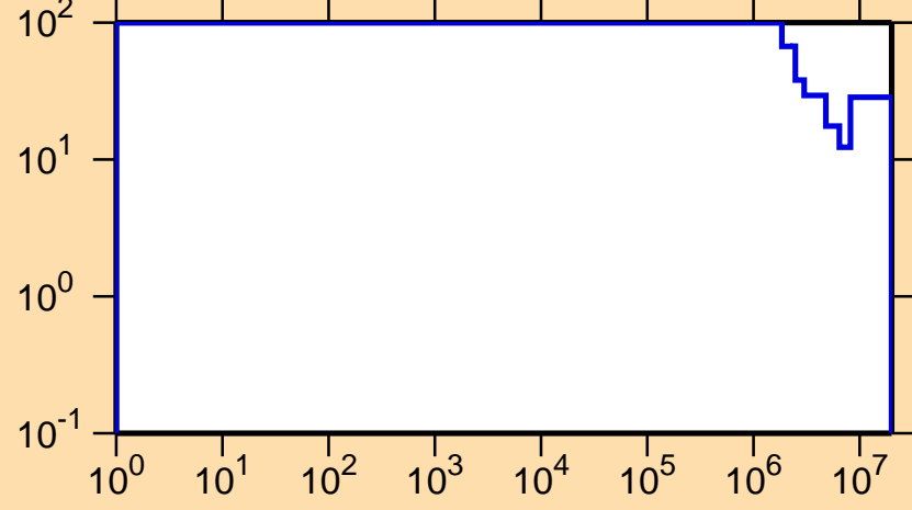
\Delta\sigma/\sigma vs. E for ^{203}\text{Po}(n,n\text{cont.})
