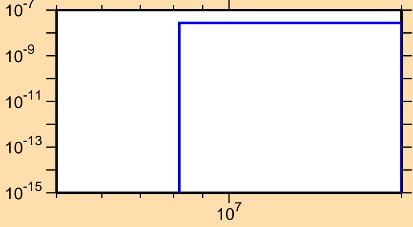
\sigma vs. E for ^{203}\text{Po}(n,2n\alpha)
