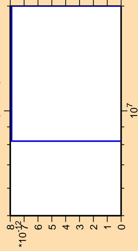
\Delta\sigma/\sigma vs. E for ^{203}\text{Po} (mt 42)
