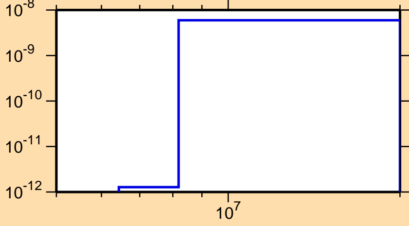
\sigma vs. E for ^{203}\text{Po}(n,p\alpha)
