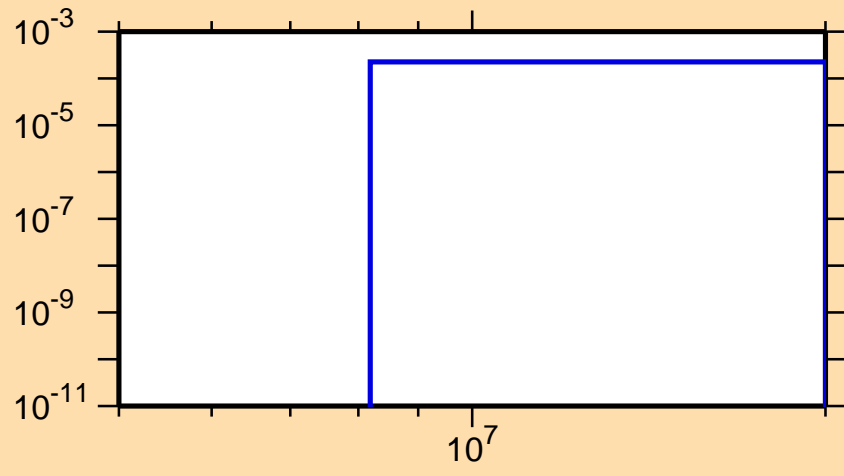
\sigma vs. E for ^{203}\text{Po}(n,t)
