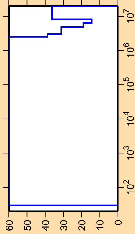
\Delta\sigma/\sigma vs. E for ^{203}\text{Po}(n,\text{inel.})
