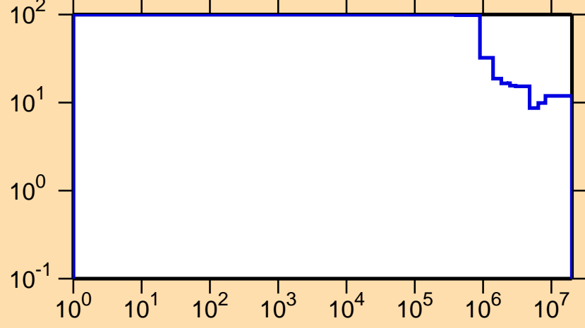
\Delta\sigma/\sigma vs. E for ^{203}\text{Po}(n,n\text{nonel.})
