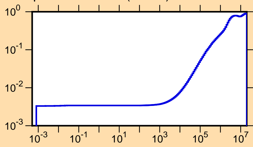
\mu vs. E for ^{204}\text{Po}(\text{mt251})
