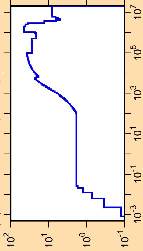
\Delta\mu/\mu vs. E for ^{204}\text{Po}(\text{mt251})
