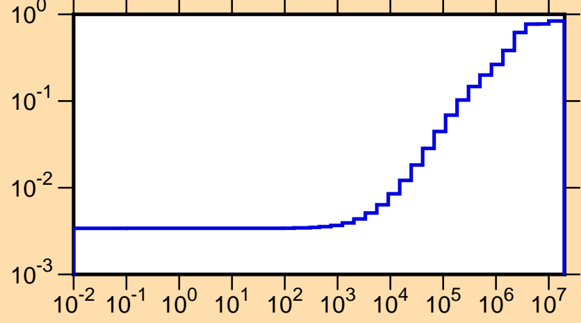
\mu vs. E for ^{204}\text{Po}(\text{mt251})
