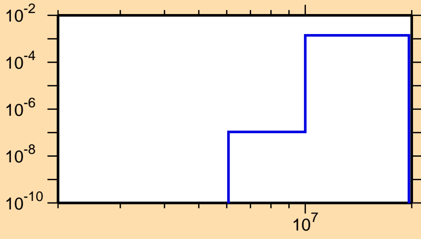
\sigma vs. E for ^{204}\text{Po}(n,d)
