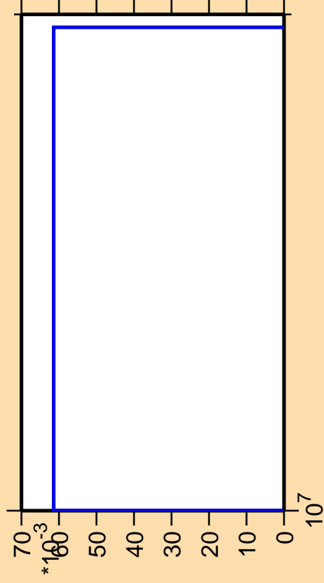
\Delta\sigma/\sigma vs. E for ^{204}\text{Po} (mt 45)
