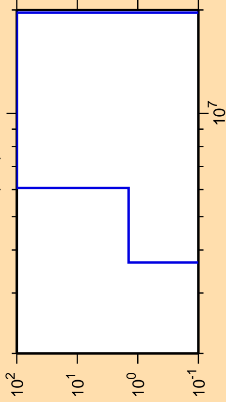
\Delta\sigma/\sigma vs. E for ^{204}\text{Po}(n,d)
