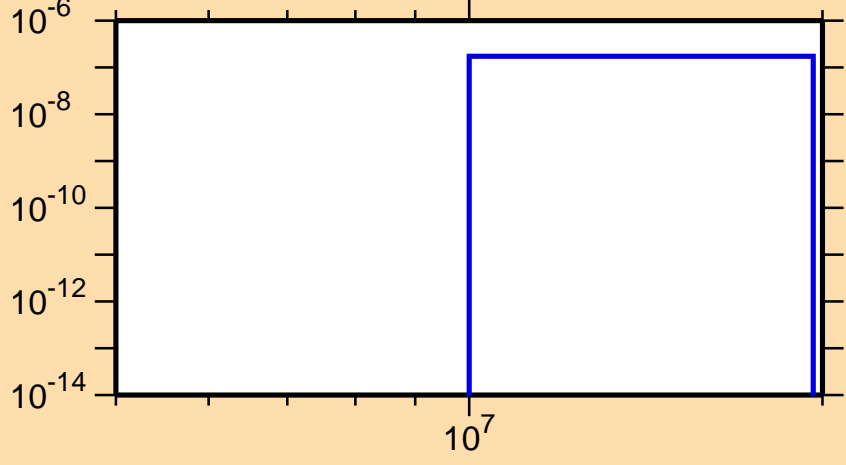
\sigma vs. E for ^{204}\text{Po}(n,2n\alpha)
