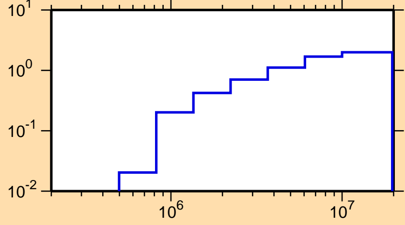
\sigma vs. E for ^{204}\text{Po}(n,\text{inel.})
