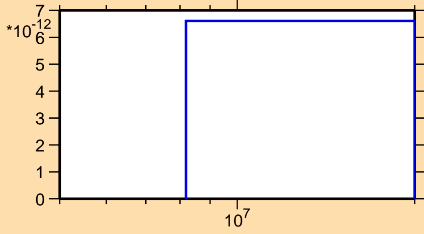
\sigma vs. E for ^{204}\text{Po}(n,\text{nt})
