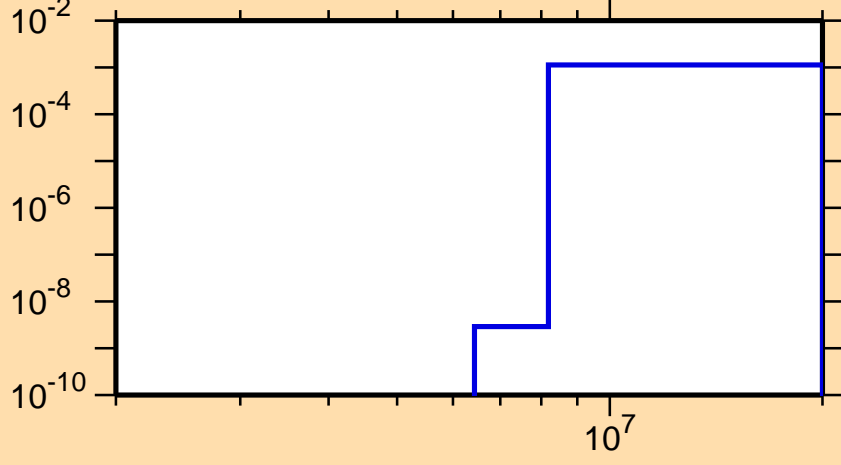
\sigma vs. E for ^{204}\text{Po}(n,d)
