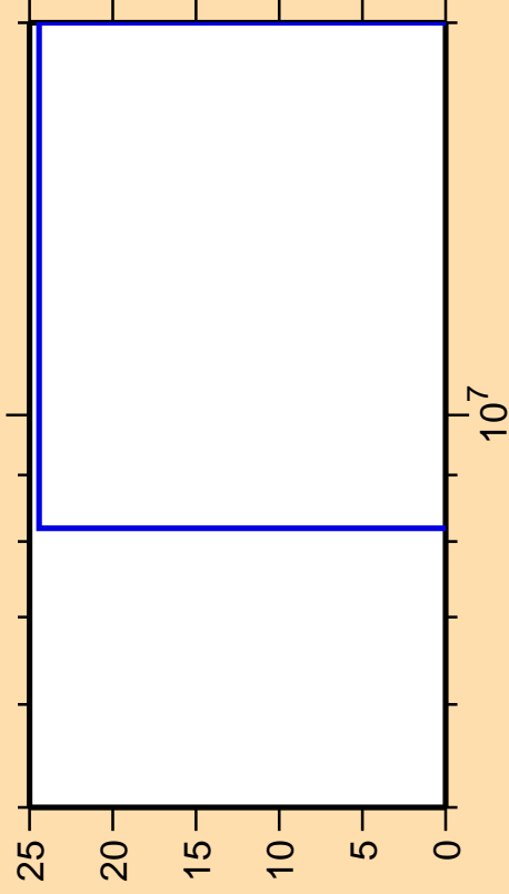
\Delta\sigma/\sigma vs. E for ^{204}\text{Po}(n,\text{nt})
