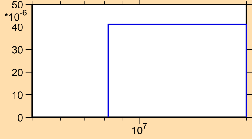
\sigma vs. E for ^{204}\text{Po}(n,t)
