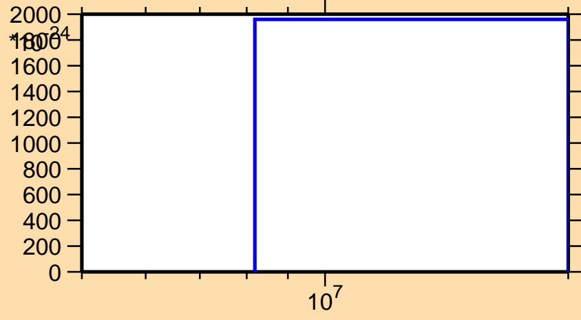
\sigma vs. E for ^{204}\text{Po}(\text{mt } 11)
