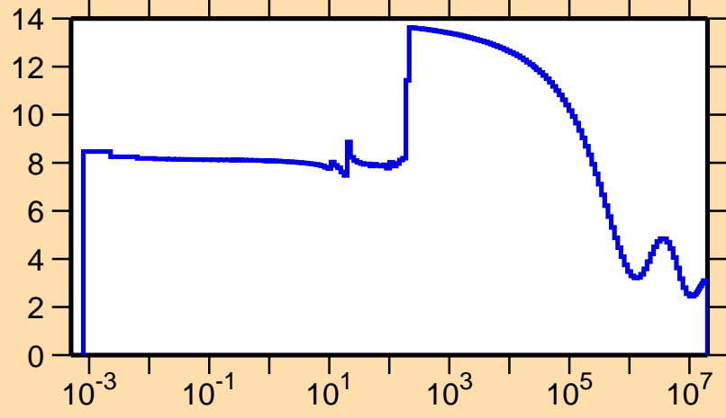
\sigma vs. E for ^{205}\text{Po}(n,\text{el.})
