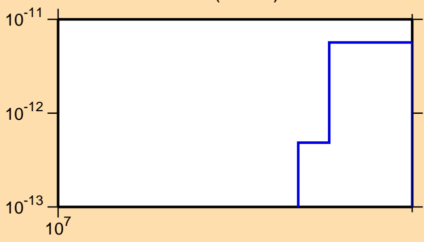
\sigma vs. E for ^{205}\text{Po} (mt 45)
