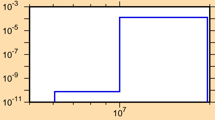
\sigma vs. E for ^{205}\text{Po}(n,t)
