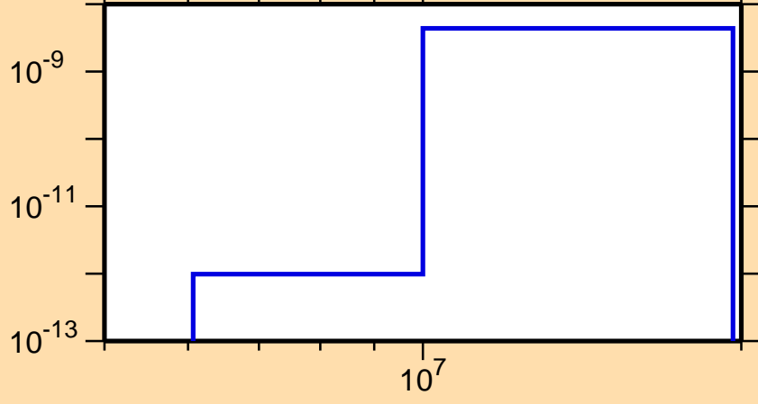
\sigma vs. E for ^{205}\text{Po}(n,p\alpha)
