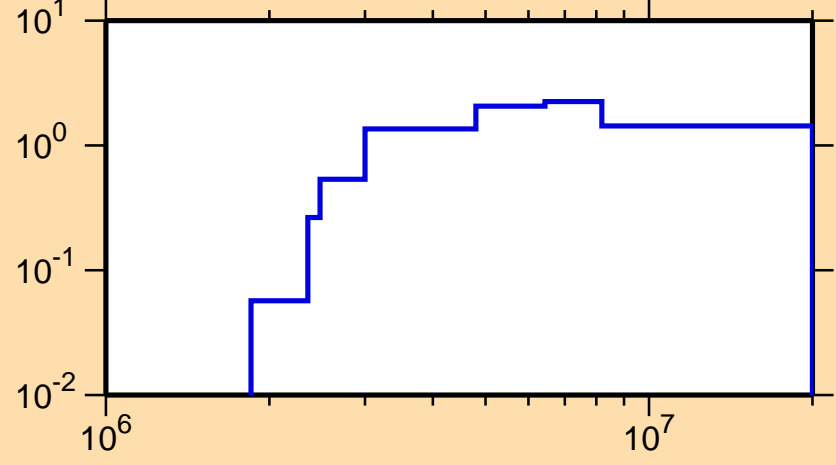
\sigma vs. E for ^{205}\text{Po}(n,n\text{cont.})
