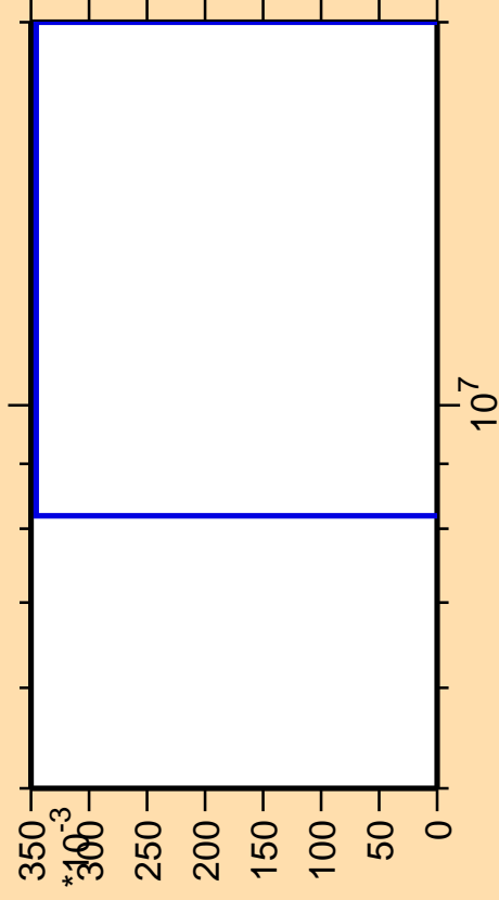
\Delta\sigma/\sigma vs. E for ^{205}\text{Po}(\text{mt } 45)
