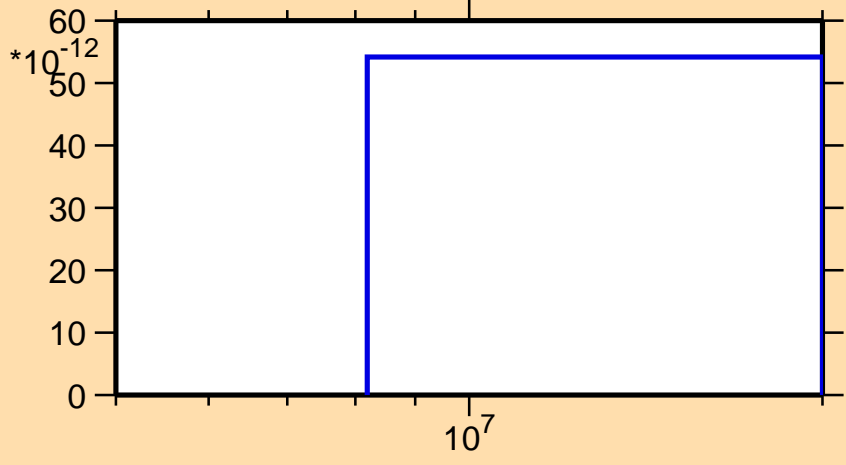
\sigma vs. E for ^{205}\text{Po}(n,\text{nt})
