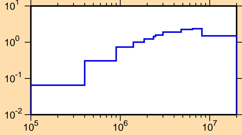
\sigma vs. E for ^{205}\text{Po}(n,\text{inel.})
