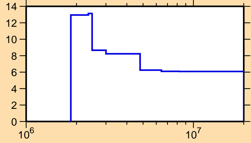
\Delta\sigma/\sigma vs. E for ^{205}\text{Po}(n,n\text{onel.})
