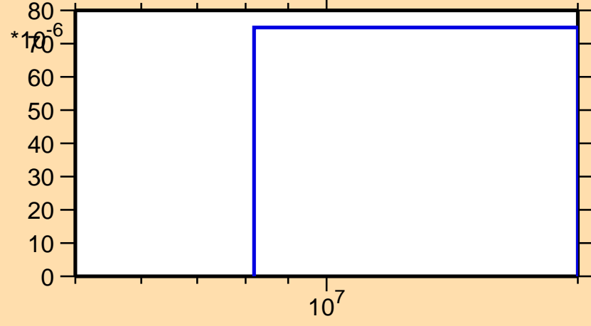
\sigma vs. E for ^{205}\text{Po}(n,3n)
