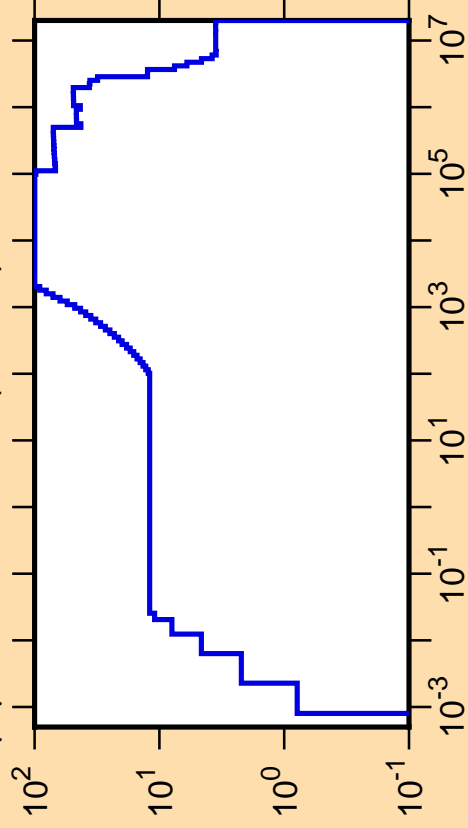
\Delta\mu/\mu vs. E for ^{206}\text{Po}(\text{mt251})
