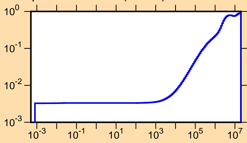
\mu vs. E for ^{206}\text{Po}(\text{mt251})
