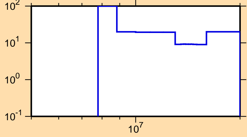
\Delta\sigma/\sigma vs. E for ^{206}\text{Po}(n,2n)
