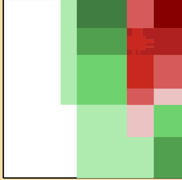
\Delta\sigma/\sigma vs. E for ^{206}\text{Po}(n,2n)
