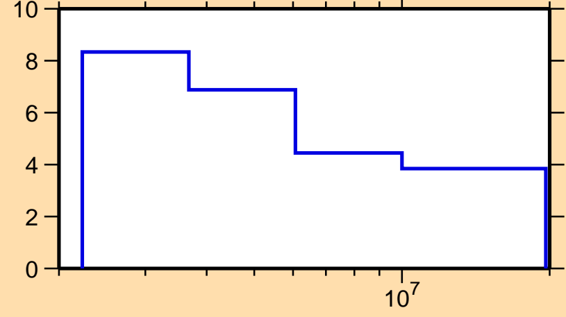
\Delta\sigma/\sigma vs. E for ^{206}\text{Po}(n,n\text{nonel.})
