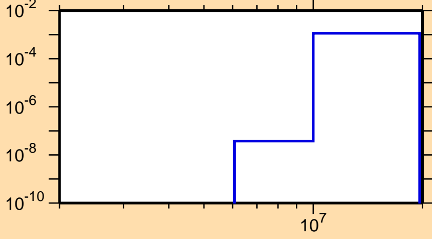
\sigma vs. E for ^{206}\text{Po}(n,d)
