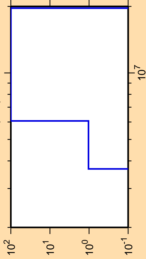
\Delta\sigma/\sigma vs. E for ^{206}\text{Po}(n,d)
