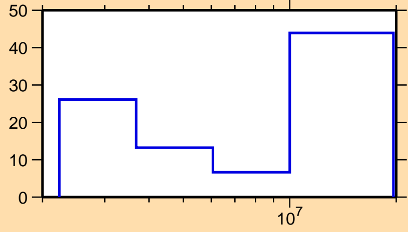
\Delta\sigma/\sigma vs. E for ^{206}\text{Po}(n,ncont.)
