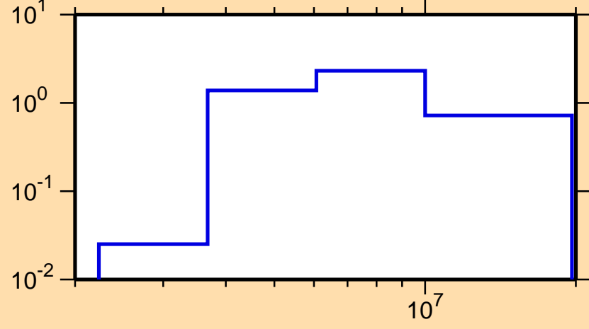
\sigma vs. E for ^{206}\text{Po}(n,n\text{cont.})
