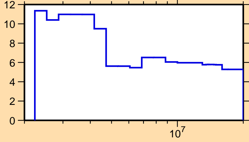
\Delta\sigma/\sigma vs. E for ^{207}\text{Po}(n,n\text{inel.})
