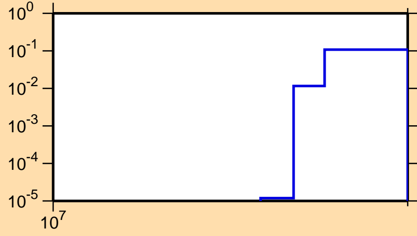
\sigma vs. E for ^{207}\text{Po}(n,3n)
