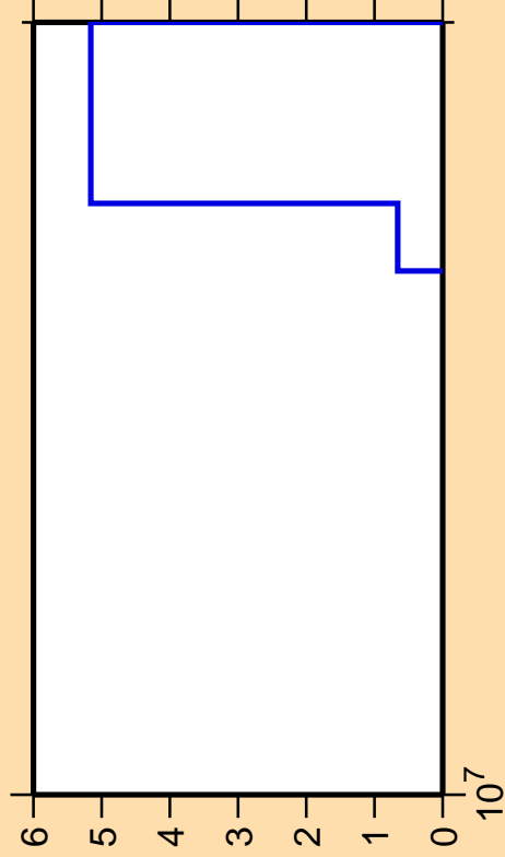
\Delta\sigma/\sigma vs. E for ^{207}\text{Po}(\text{mt117})
