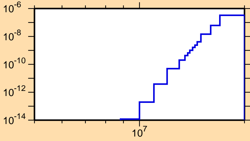
\sigma vs. E for ^{207}\text{Po}(n,\text{He}3)
