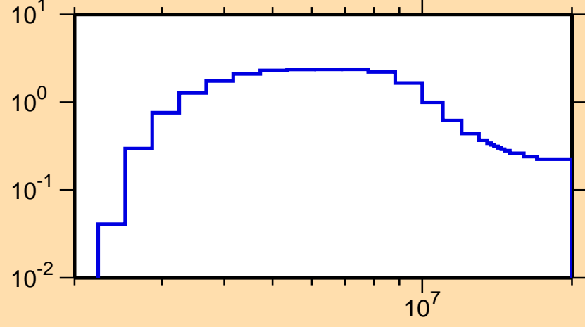
\sigma vs. E for ^{207}\text{Po}(n,n\text{cont.})
