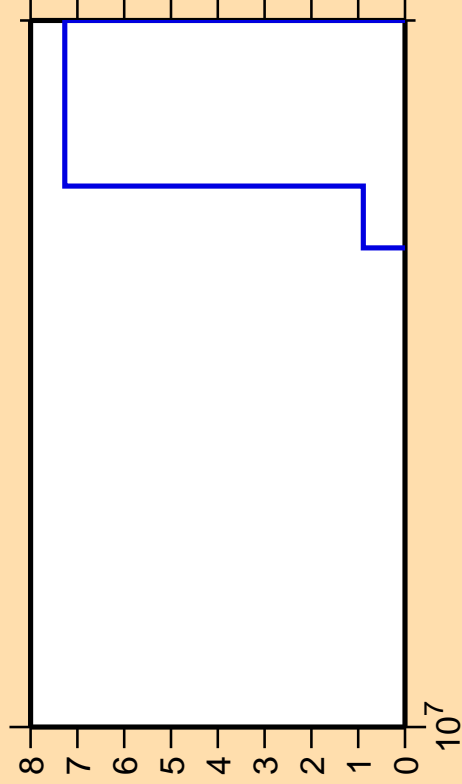
\Delta\sigma/\sigma vs. E for ^{207}\text{Po} (mt 45)
