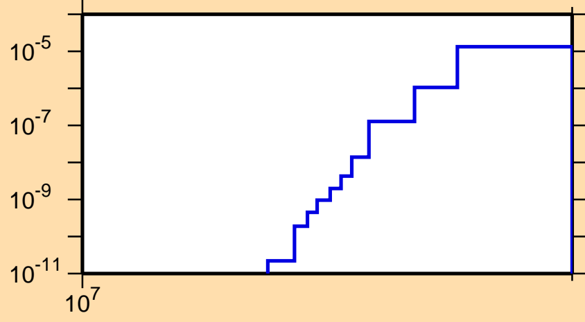
\sigma vs. E for ^{207}\text{Po}(n,\text{nd})
