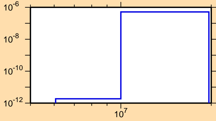
\sigma vs. E for ^{207}\text{Po}(n,p\alpha)
