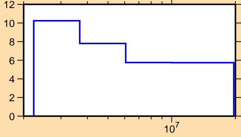
\Delta\sigma/\sigma vs. E for ^{207}\text{Po}(n,n\text{nonel.})
