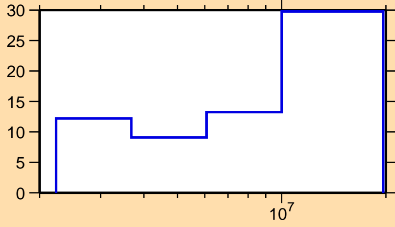
\Delta\sigma/\sigma vs. E for ^{207}\text{Po}(n,ncont.)
