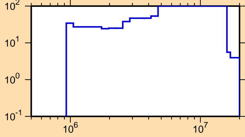
\Delta\sigma/\sigma vs. E for ^{207}\text{Po}(n,n_1)
