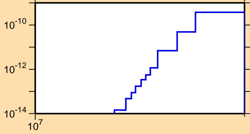
\sigma vs. E for ^{207}\text{Po}(n,\text{pd})
