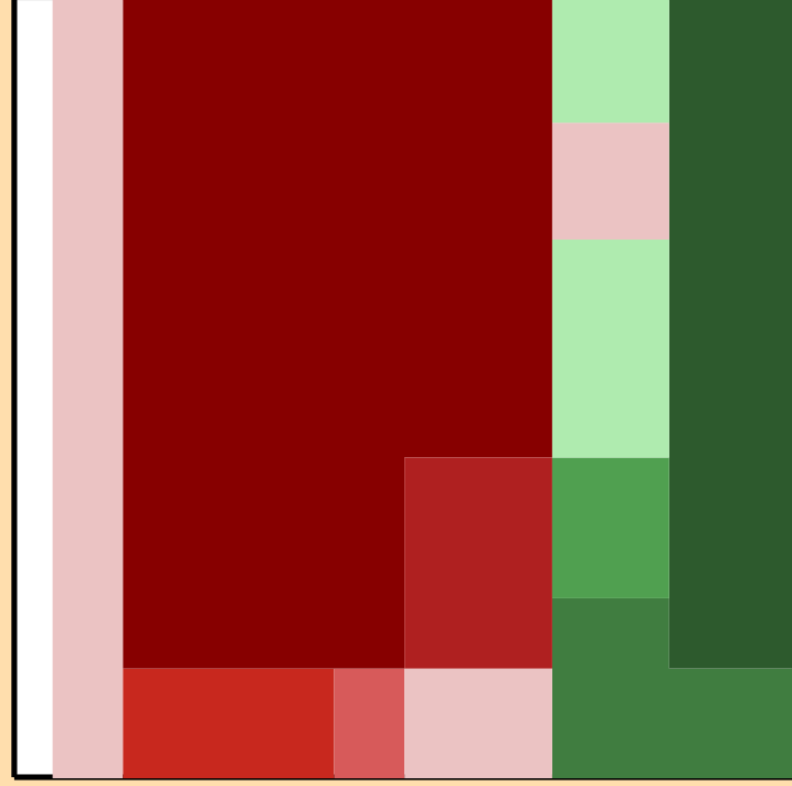
\Delta\sigma/\sigma vs. E for ^{207}\text{Po}(n,2n)
