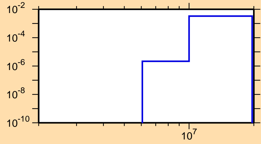
\sigma vs. E for ^{207}\text{Po}(n,d)
