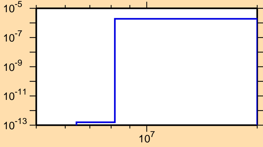
\sigma vs. E for ^{207}\text{Po}(n,2n\alpha)
