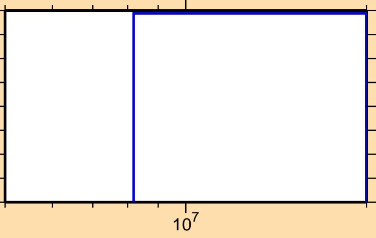
\sigma vs. E for ^{207}\text{Po}(n,2np)
