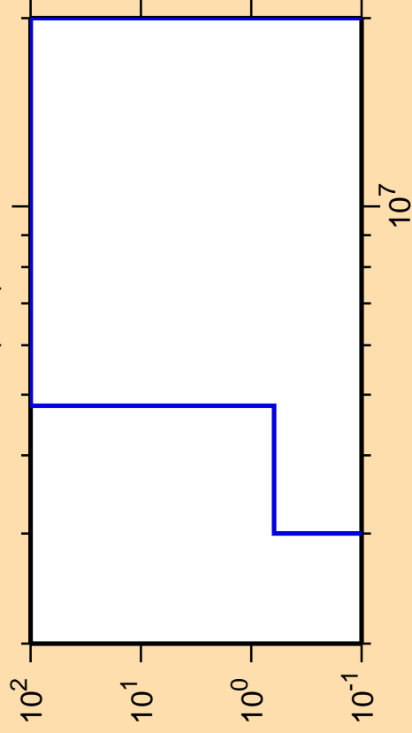
\Delta\sigma/\sigma vs. E for ^{207}\text{Po}(n,d)
