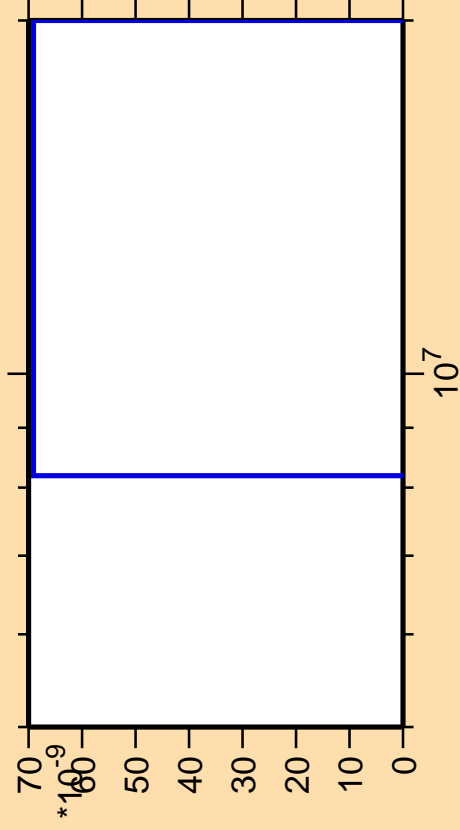
\Delta\sigma/\sigma vs. E for ^{207}\text{Po} (mt 42)
