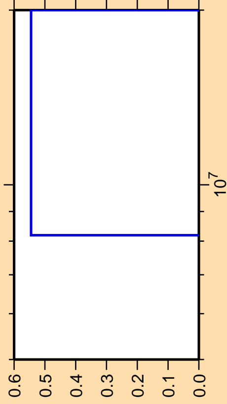
\Delta\sigma/\sigma vs. E for ^{207}\text{Po} (mt 45)
