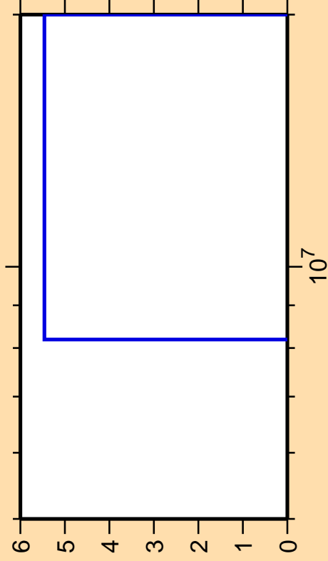
\Delta\sigma/\sigma vs. E for ^{207}\text{Po}(\text{mt } 34)
