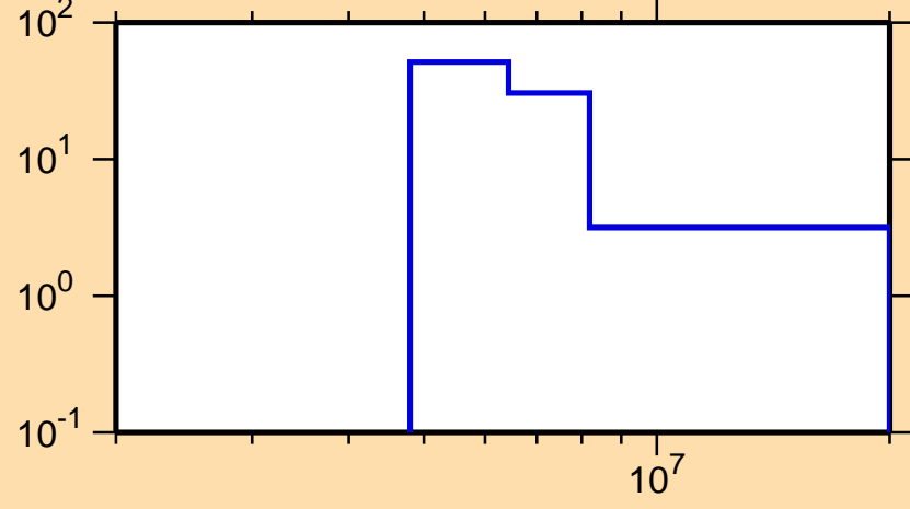
\Delta\sigma/\sigma vs. E for ^{207}\text{Po}(n,2n)
