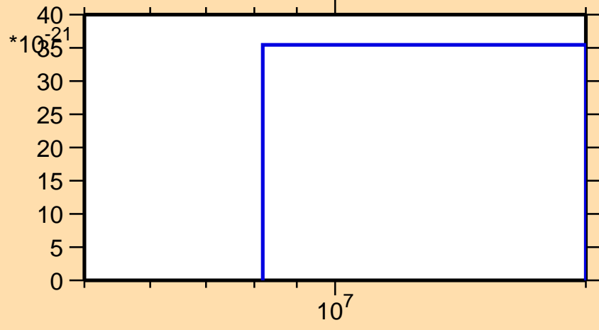
\sigma vs. E for ^{207}\text{Po} (mt 42)
