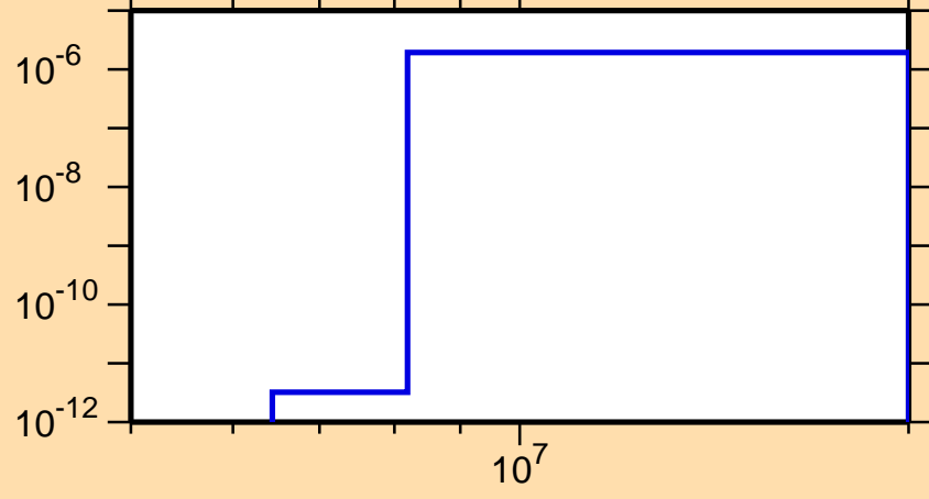
\sigma vs. E for ^{207}\text{Po}(n,p\alpha)
