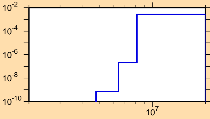
\sigma vs. E for ^{207}\text{Po}(n,d)
