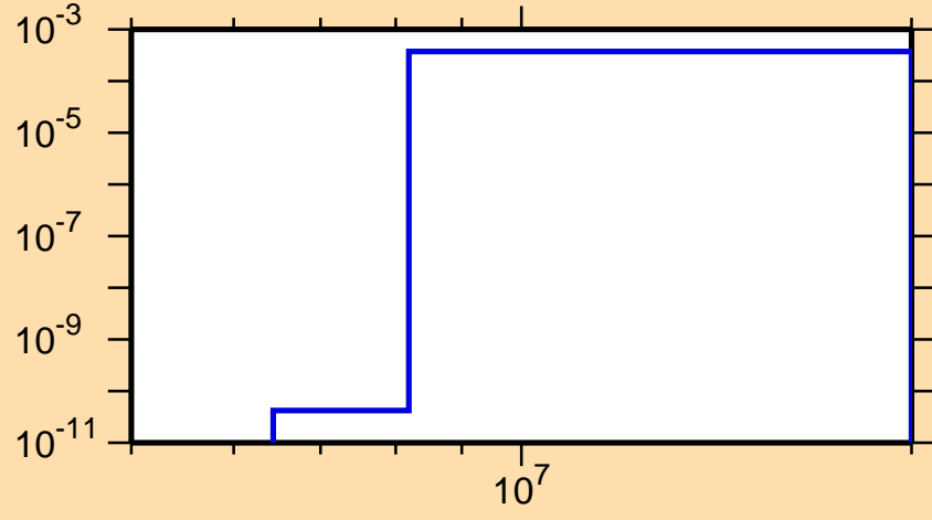
\sigma vs. E for ^{207}\text{Po}(n,t)
