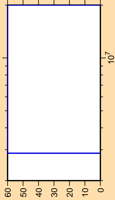
\Delta\sigma/\sigma vs. E for ^{208}\text{Po}(n,\gamma)
