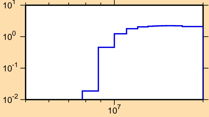
\sigma vs. E for ^{208}\text{Po}(n,2n)
