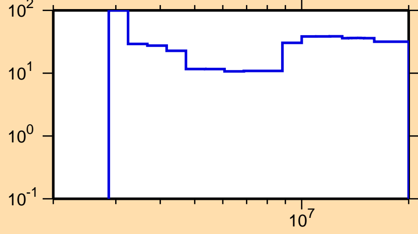
\Delta\sigma/\sigma vs. E for ^{208}\text{Po}(n,n\text{cont.})
