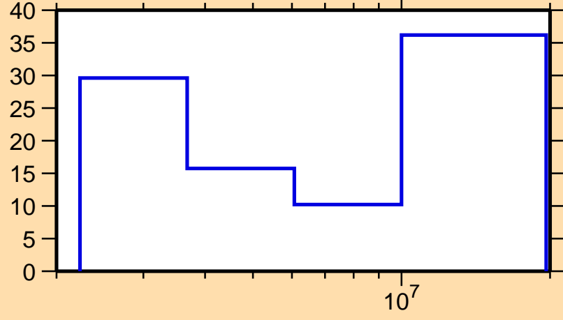
\Delta\sigma/\sigma vs. E for ^{208}\text{Po}(n,ncont.)
