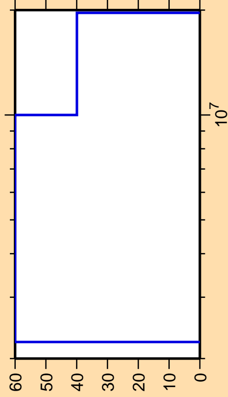
\Delta\sigma/\sigma vs. E for ^{208}\text{Po}(n,p)
