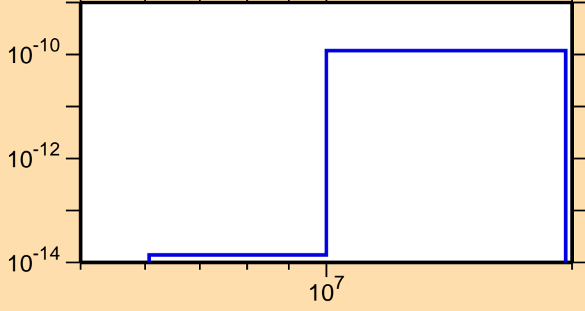
\sigma vs. E for ^{208}\text{Po}(n,p\alpha)
