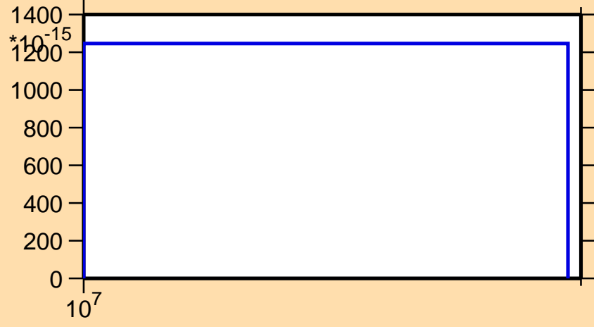
\sigma vs. E for ^{208}\text{Po} (mt 45)
