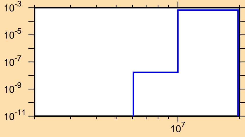
\sigma vs. E for ^{208}\text{Po}(n,d)
