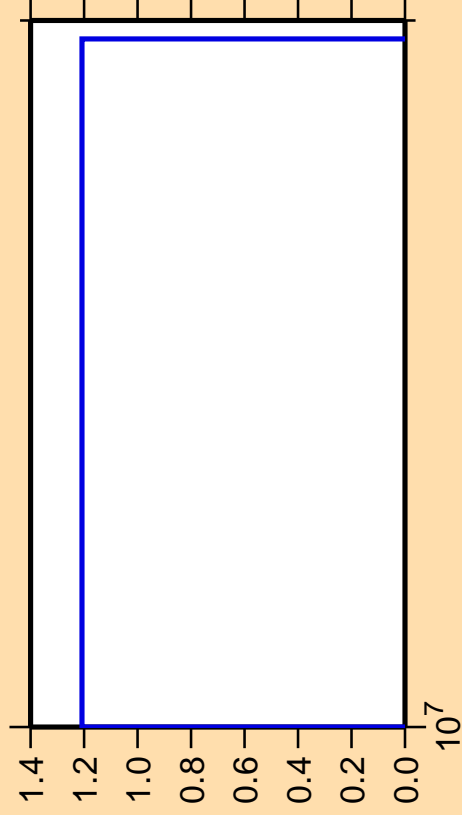
\Delta\sigma/\sigma vs. E for ^{208}\text{Po} (mt 45)
