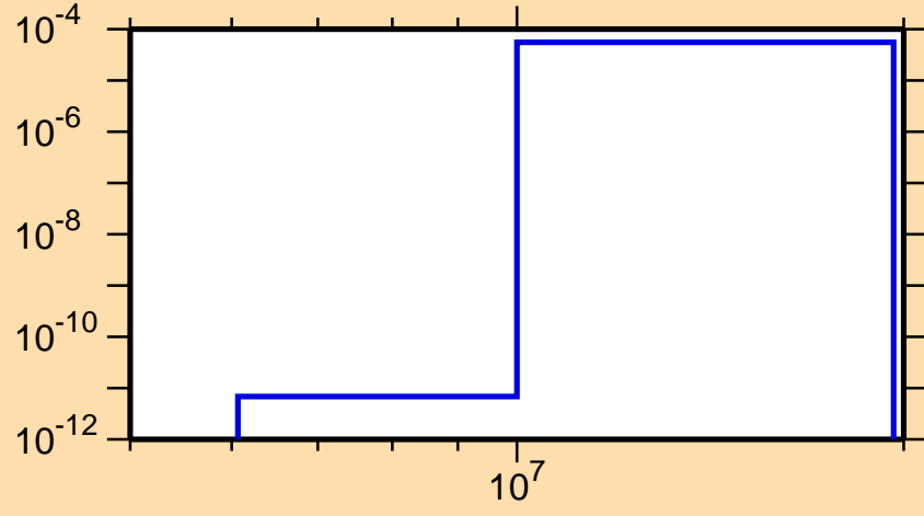
\sigma vs. E for ^{208}\text{Po}(n,t)
