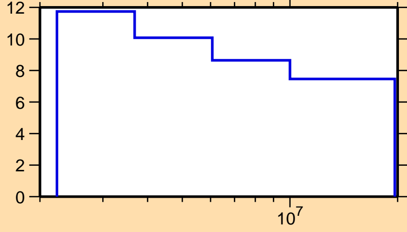
\Delta\sigma/\sigma vs. E for ^{208}\text{Po}(n,n\text{nonel.})
