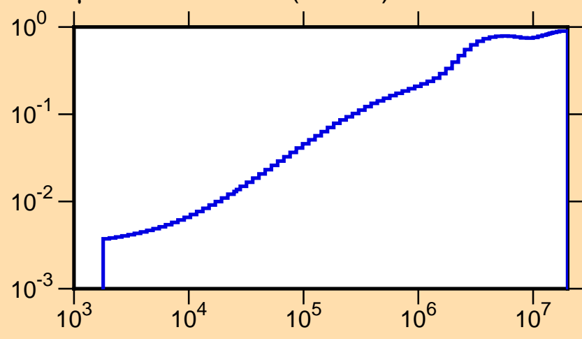
\mu vs. E for ^{209}\text{Po}(\text{mt251})
