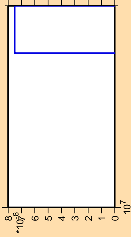
\Delta\sigma/\sigma vs. E for ^{209}\text{Po} (mt 42)
