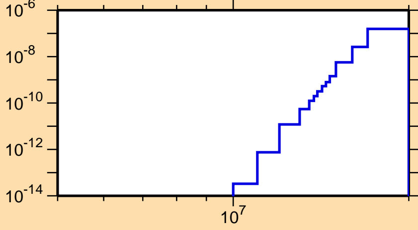
\sigma vs. E for ^{209}\text{Po}(n,\text{He3})
