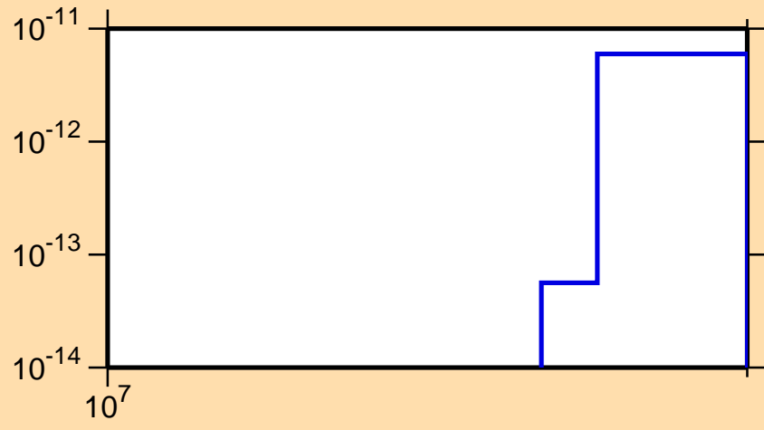
\sigma vs. E for ^{209}\text{Po} (mt 34)
