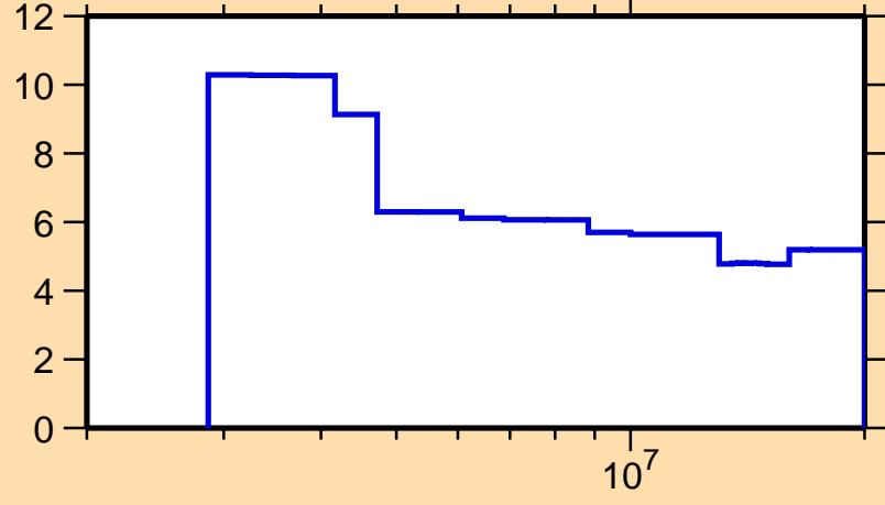
\Delta\sigma/\sigma vs. E for ^{209}\text{Po}(n,n\text{nonel.})
