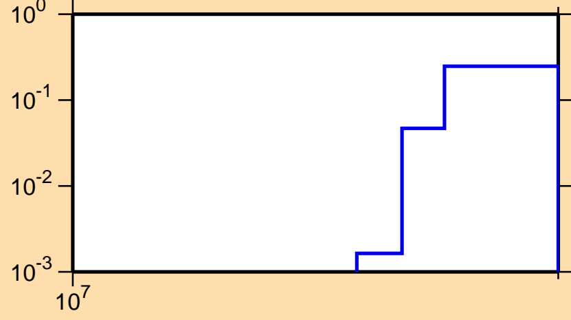
\sigma vs. E for ^{209}\text{Po}(n,3n)
