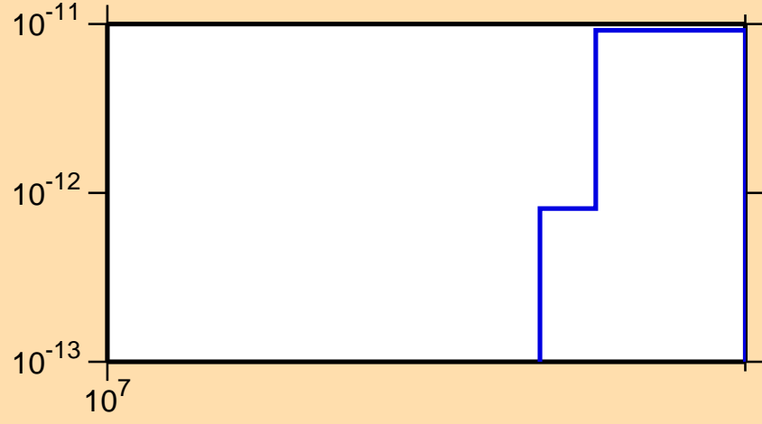
\sigma vs. E for ^{209}\text{Po}(n,3n\alpha)
