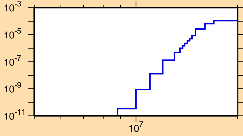
\sigma vs. E for ^{209}\text{Po}(n,2n\alpha)
