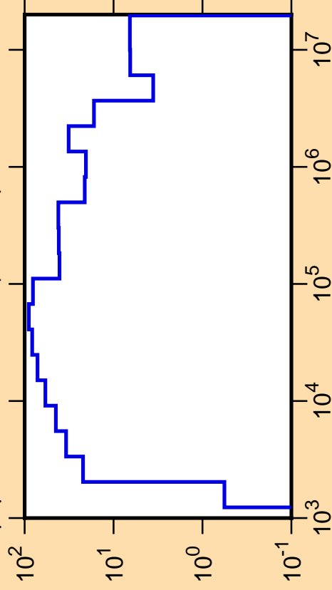
\Delta\mu/\mu vs. E for ^{209}\text{Po}(\text{mt251})
