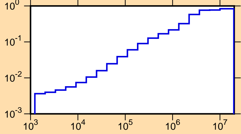
\mu vs. E for ^{209}\text{Po}(\text{mt251})
