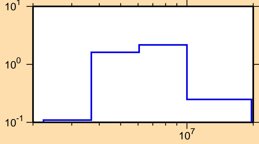
\sigma vs. E for ^{209}\text{Po}(n,n\text{cont.})
