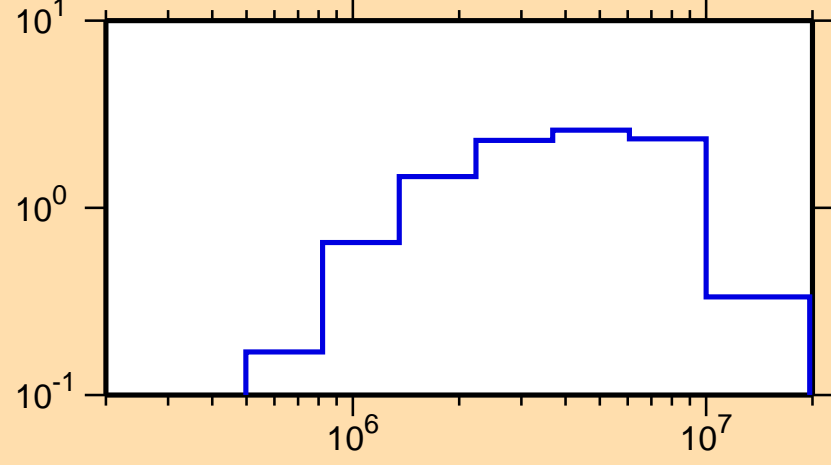
\sigma vs. E for ^{209}\text{Po}(n,\text{inel.})
