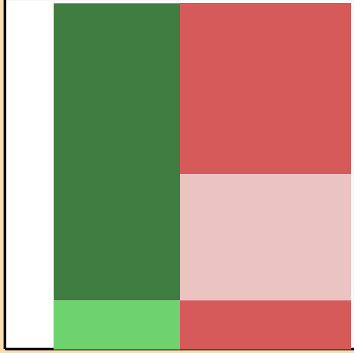
\Delta\sigma/\sigma vs. E for ^{209}\text{Po}(n,2n)
