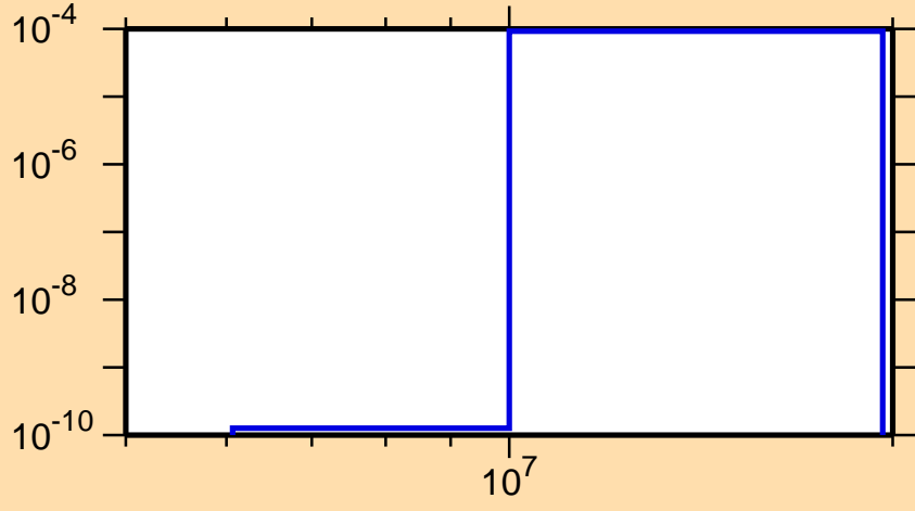
\sigma vs. E for ^{209}\text{Po}(n,t)
