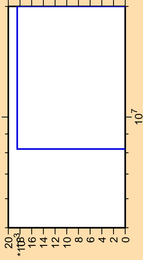
\Delta\sigma/\sigma vs. E for ^{209}\text{Po} (mt 45)
