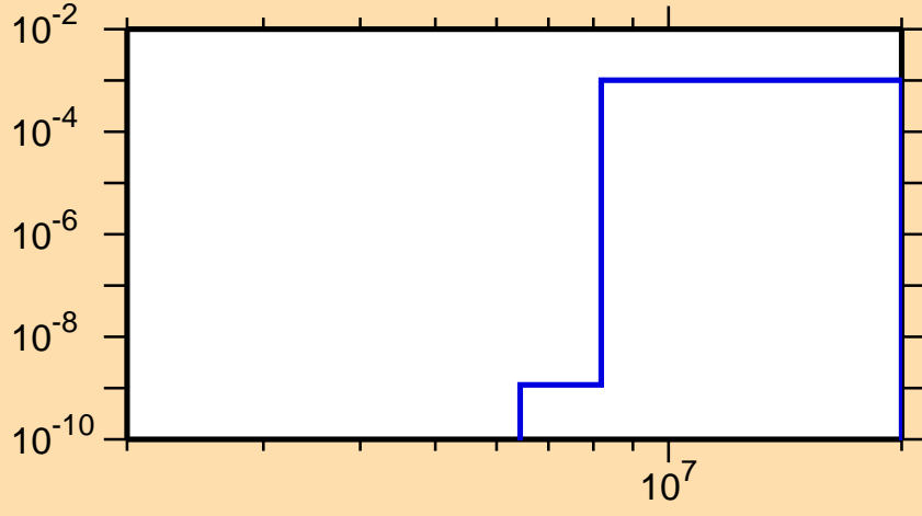
\sigma vs. E for ^{209}\text{Po}(n,d)
