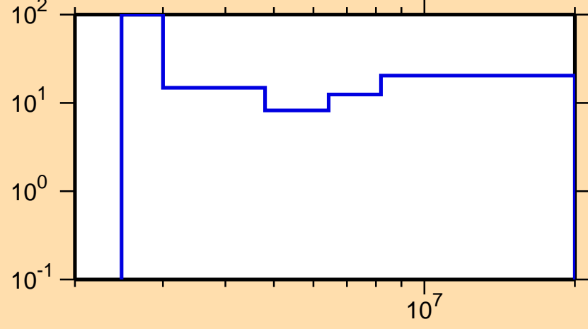
\Delta\sigma/\sigma vs. E for ^{209}\text{Po}(n,n\text{cont.})
