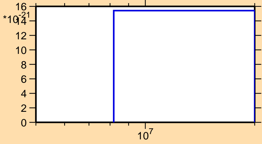
\sigma vs. E for ^{209}\text{Po} (mt 42)
