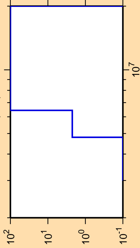
\Delta\sigma/\sigma vs. E for ^{209}\text{Po}(n,d)
