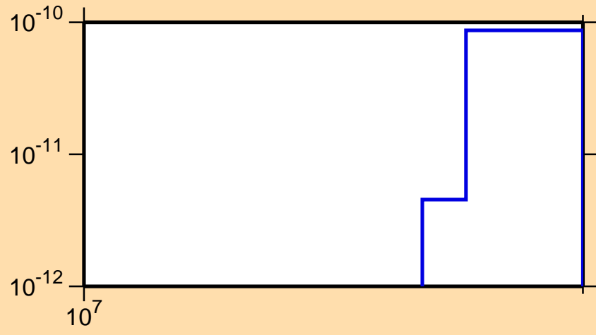
\sigma vs. E for ^{210}\text{Po}(n,\text{pd})
