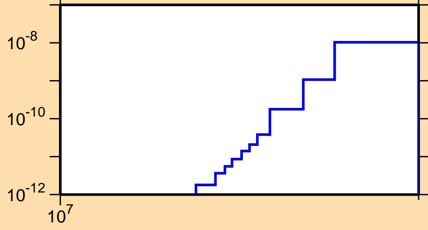
\sigma vs. E for ^{210}\text{Po}(n,\text{He}3)
