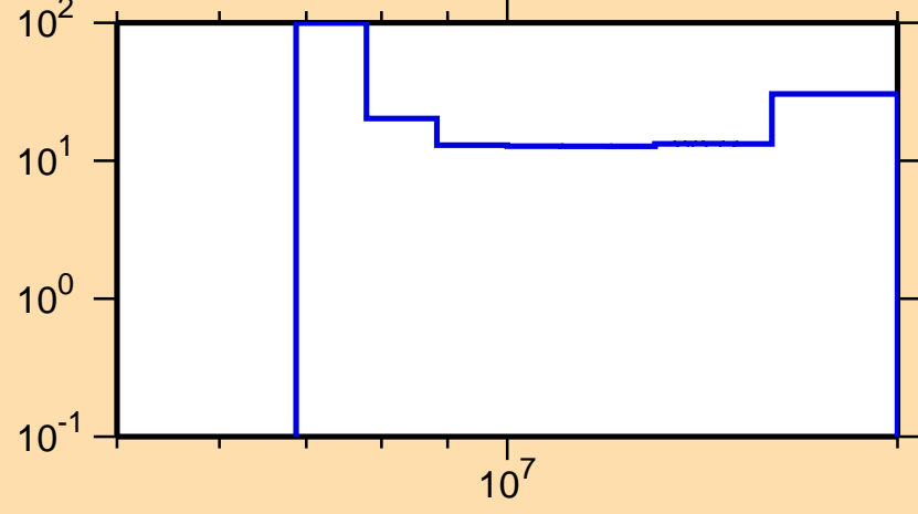
\Delta\sigma/\sigma vs. E for ^{210}\text{Po}(n,2n)
